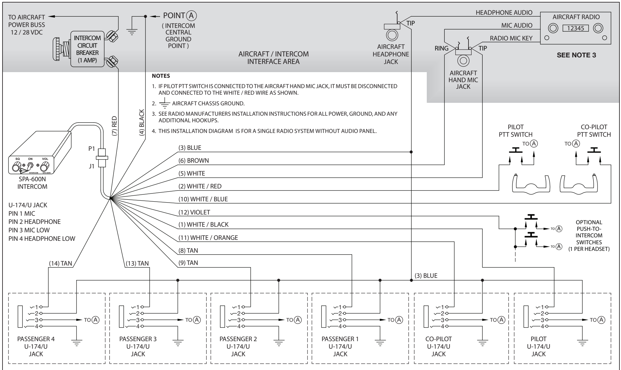
SPA-600N With U-174/U Jacks Installation Wiring Diagram
