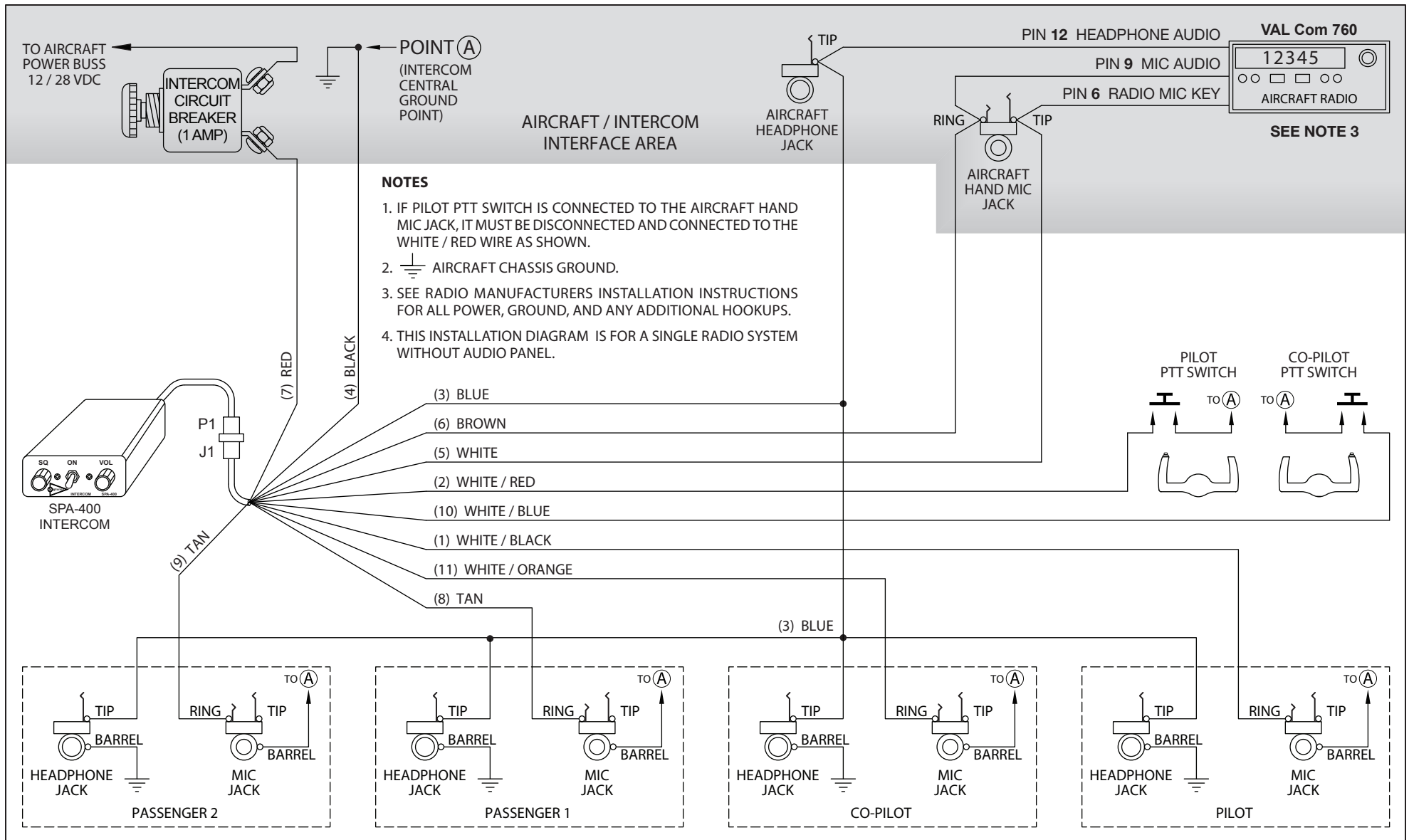
SPA-400 - VAL Com 760 Radio Installation Wiring Diagram
