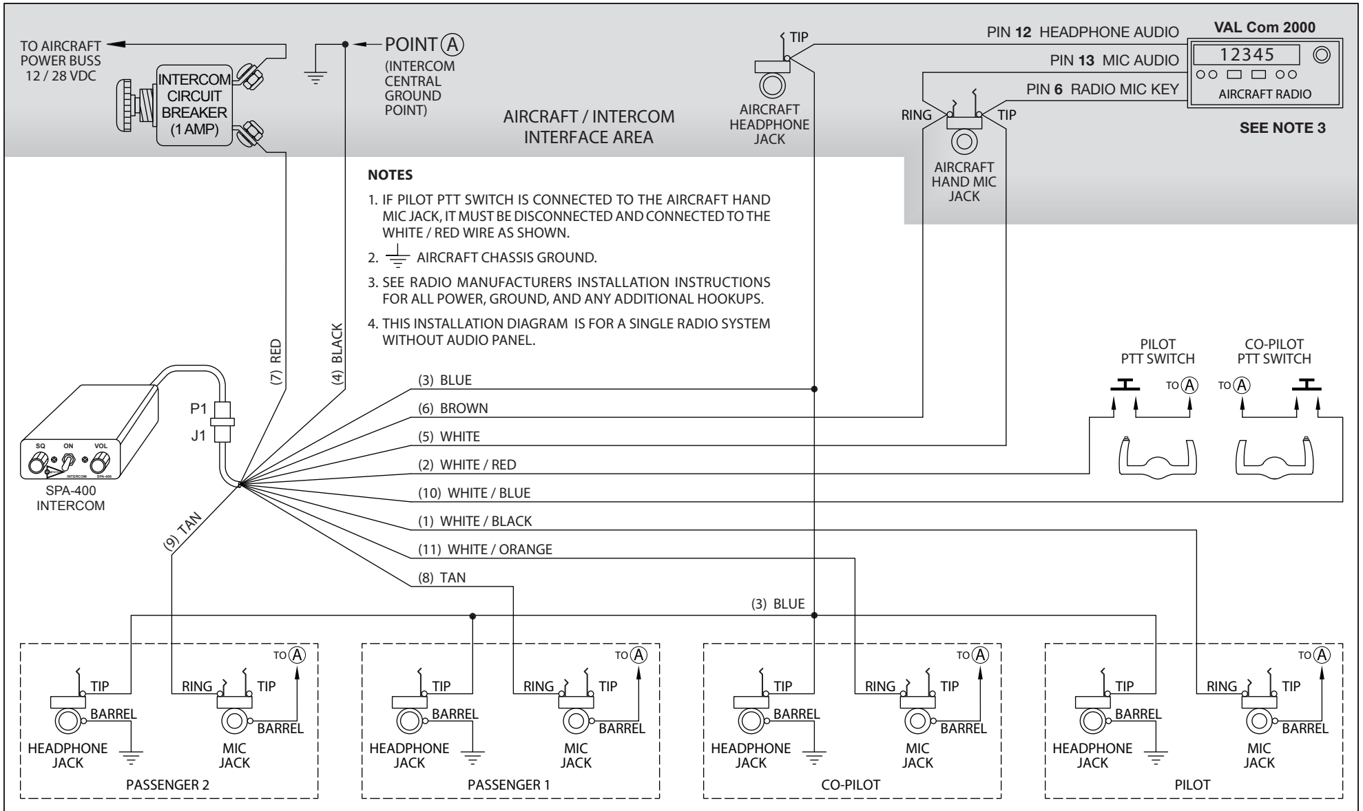
SPA-400 – VAL Com 2000 Radio Installation Wiring Diagram
