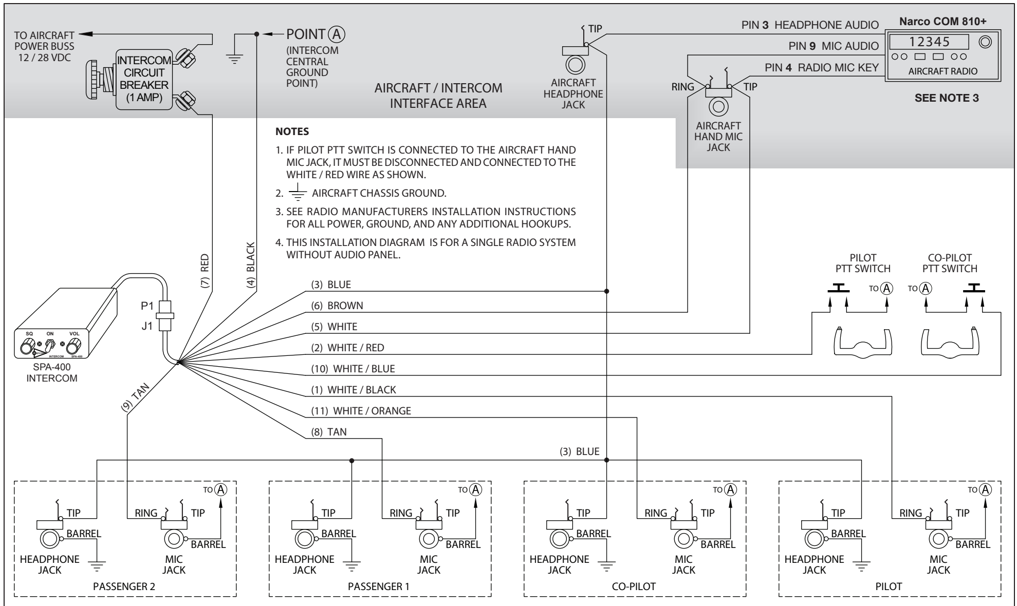
SPA-400 - Narco COM 810+ Radio Installation Wiring Diagram
