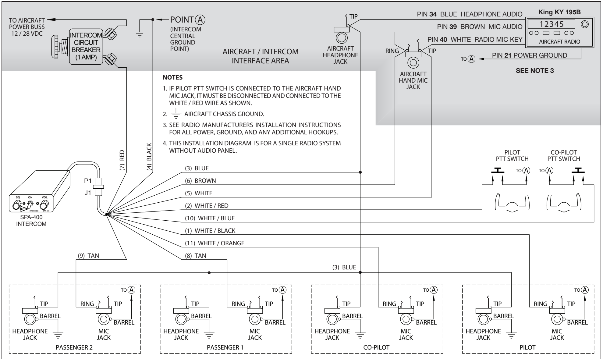
SPA-400 – King KY 195B Radio Installation Wiring Diagram
