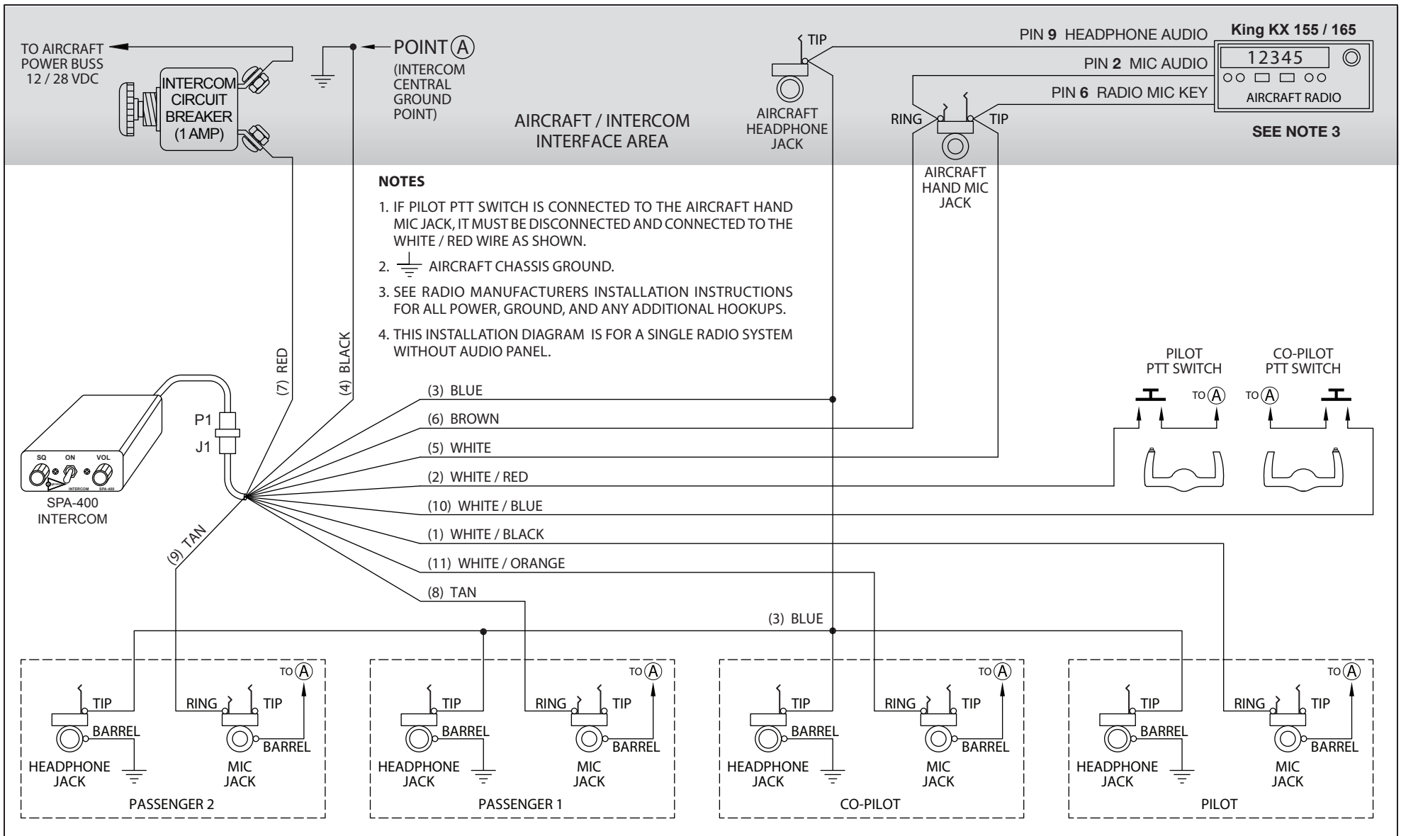
SPA-400 – King KX 155 / 165 Radio Installation Wiring Diagram
