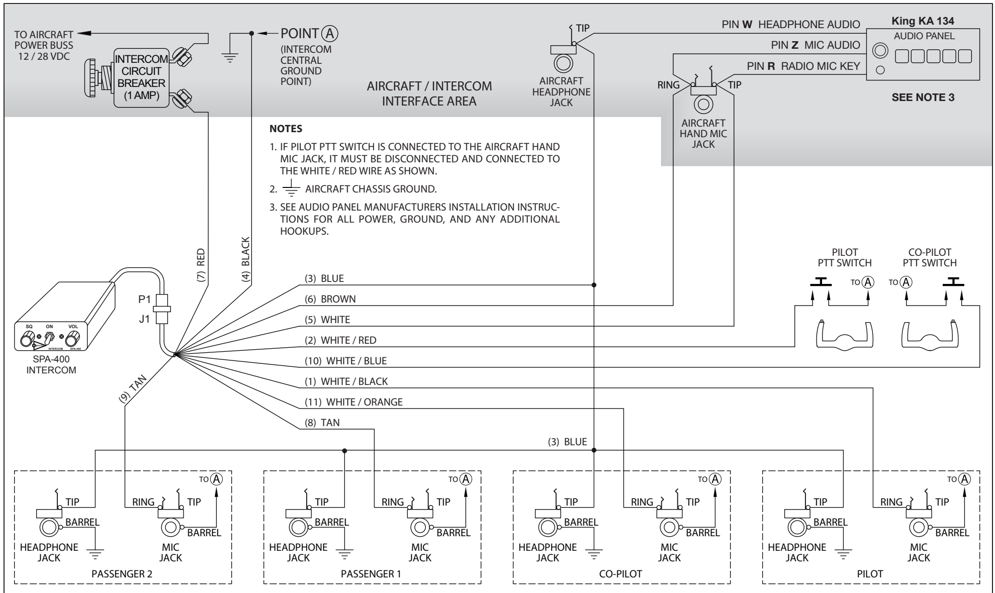
SPA-400 - King KA 134 Audio Panel Installation Wiring Diagram
