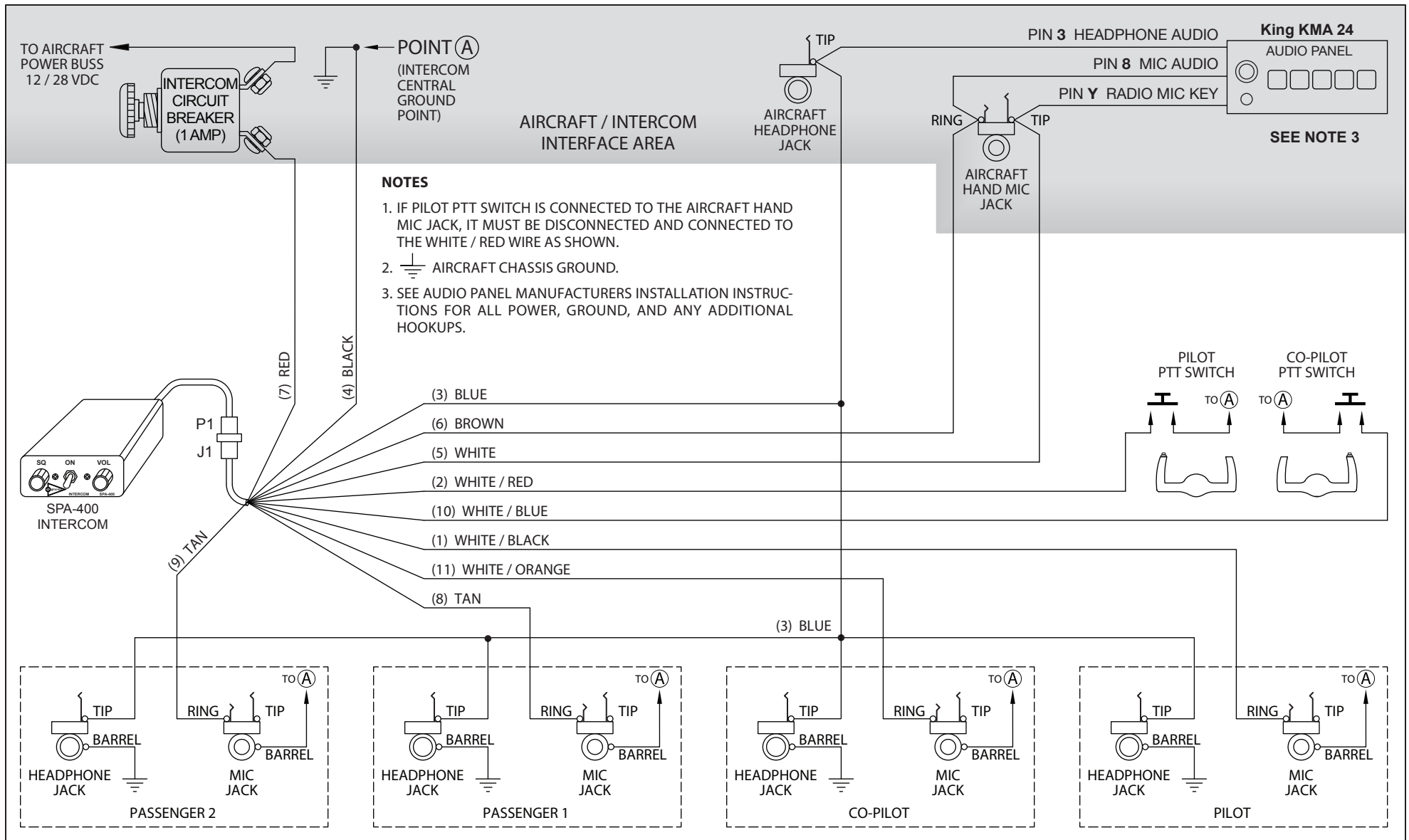
SPA-400 – King KMA 24 Audio Panel Installation Wiring Diagram
