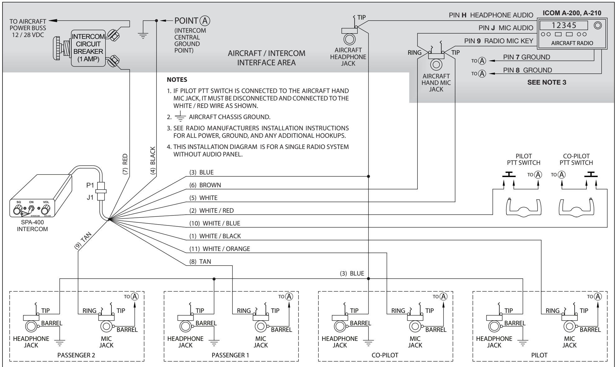
SPA-400 – ICOM A-200, A-210 Radio Installation Wiring Diagram
