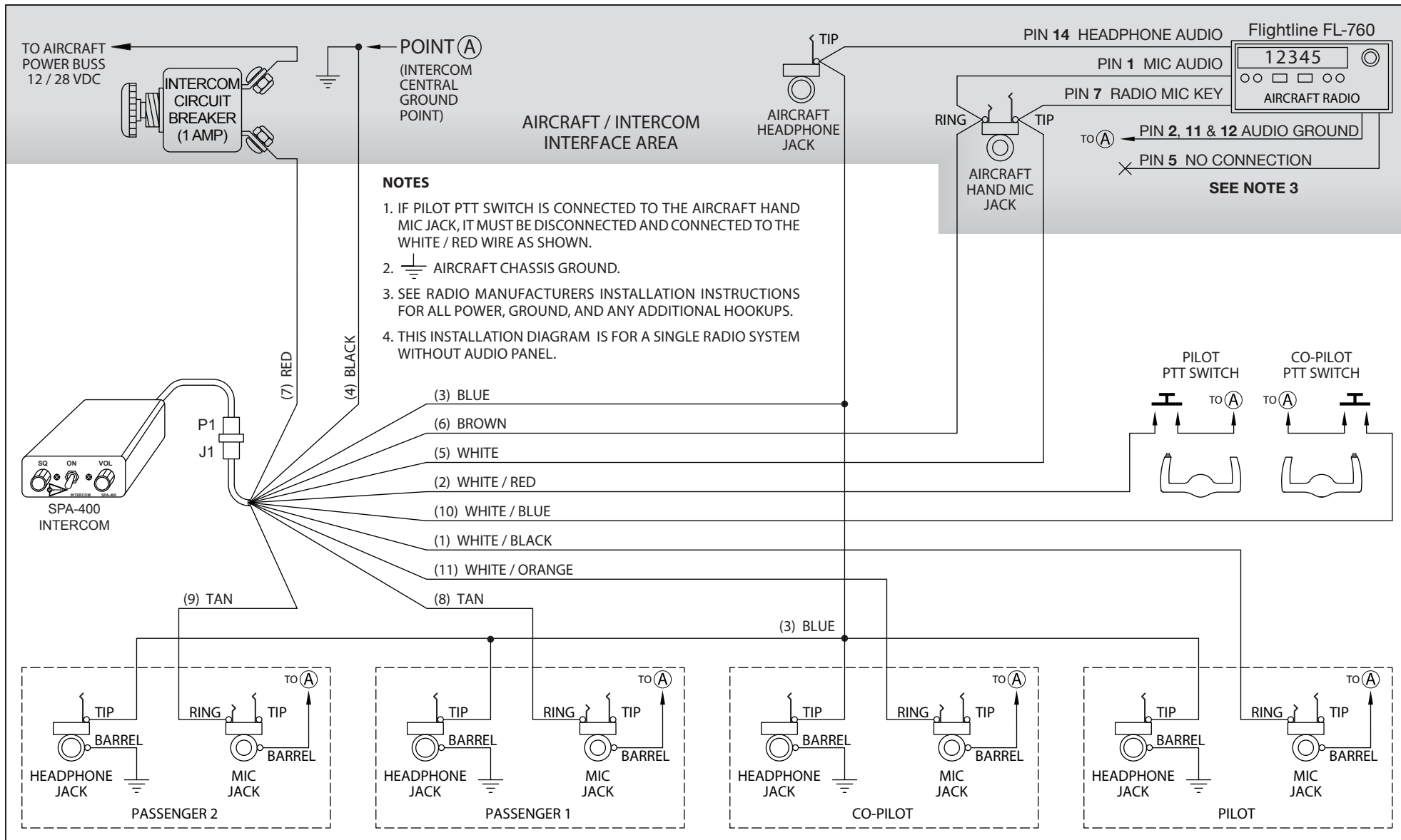
SPA-400 - Flightline FL-760 Radio Installation Wiring Diagram
