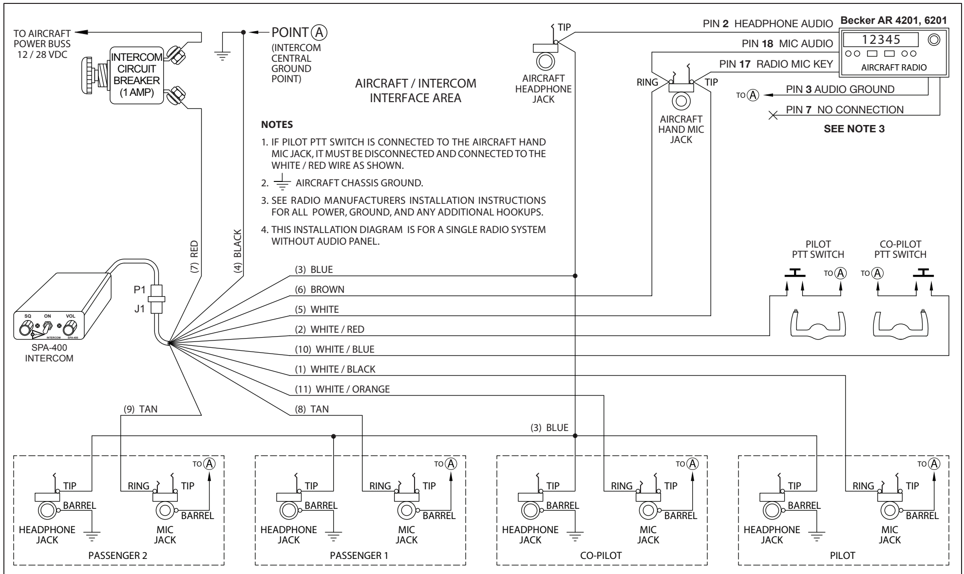
SPA-400 – Becker AR 4201, 6201 Radio Installation Wiring Diagram
