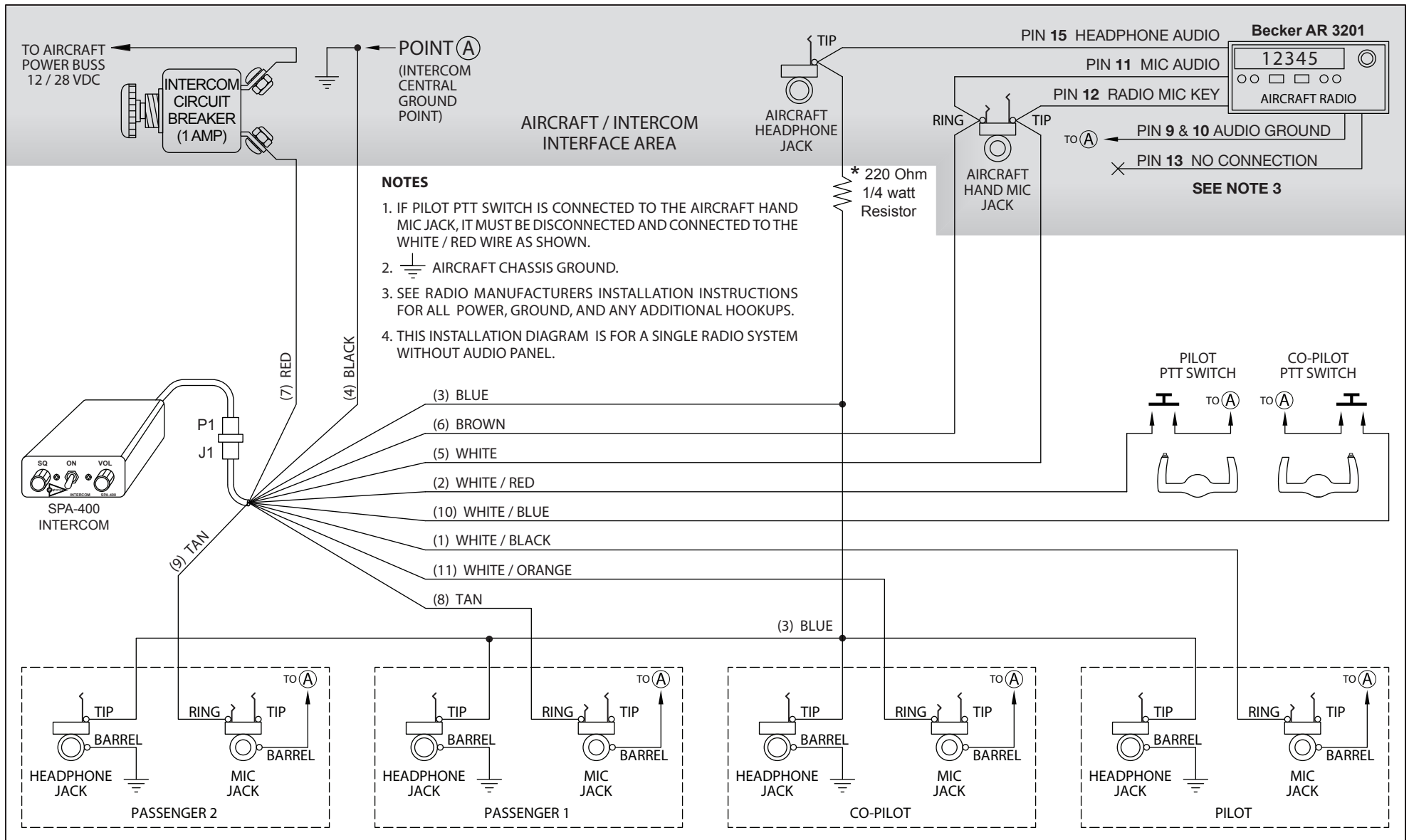
SPA-400 – Becker AR 3201 Radio Installation Wiring Diagram
