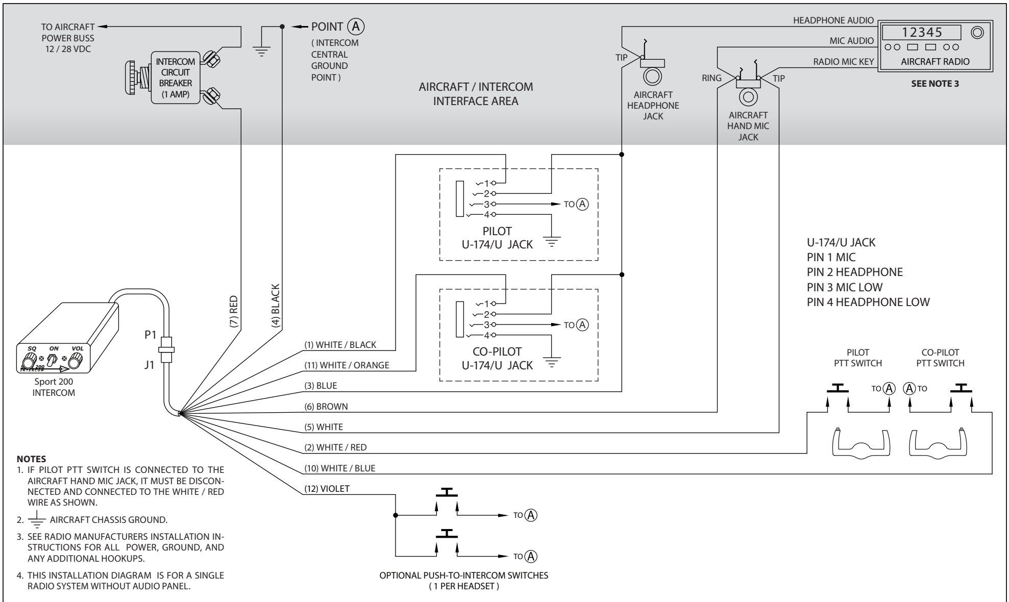
Sport 200 With U-174/U Jacks Installation Wiring Diagram
