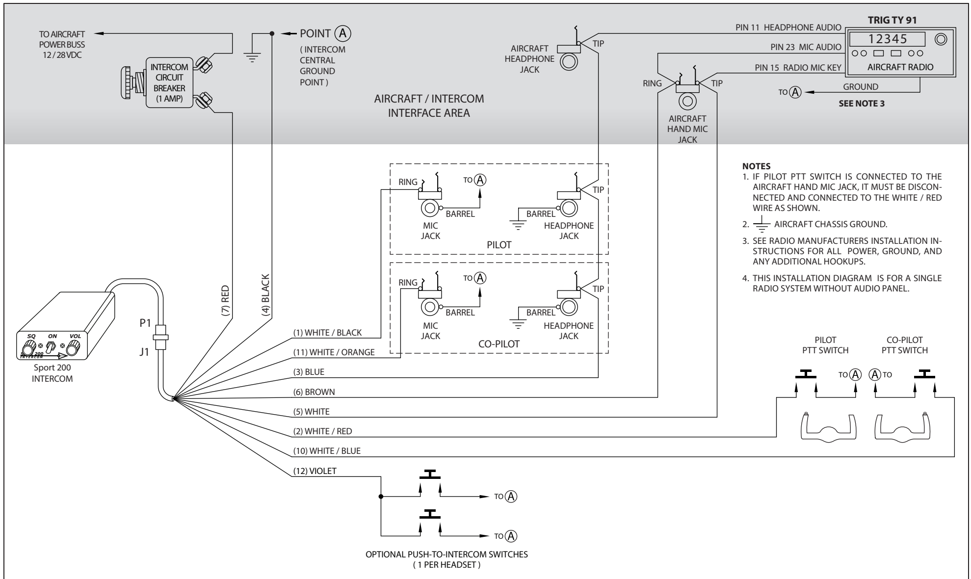
Sport 200 – TRIG TY 91 Radio Installation Wiring Diagram
