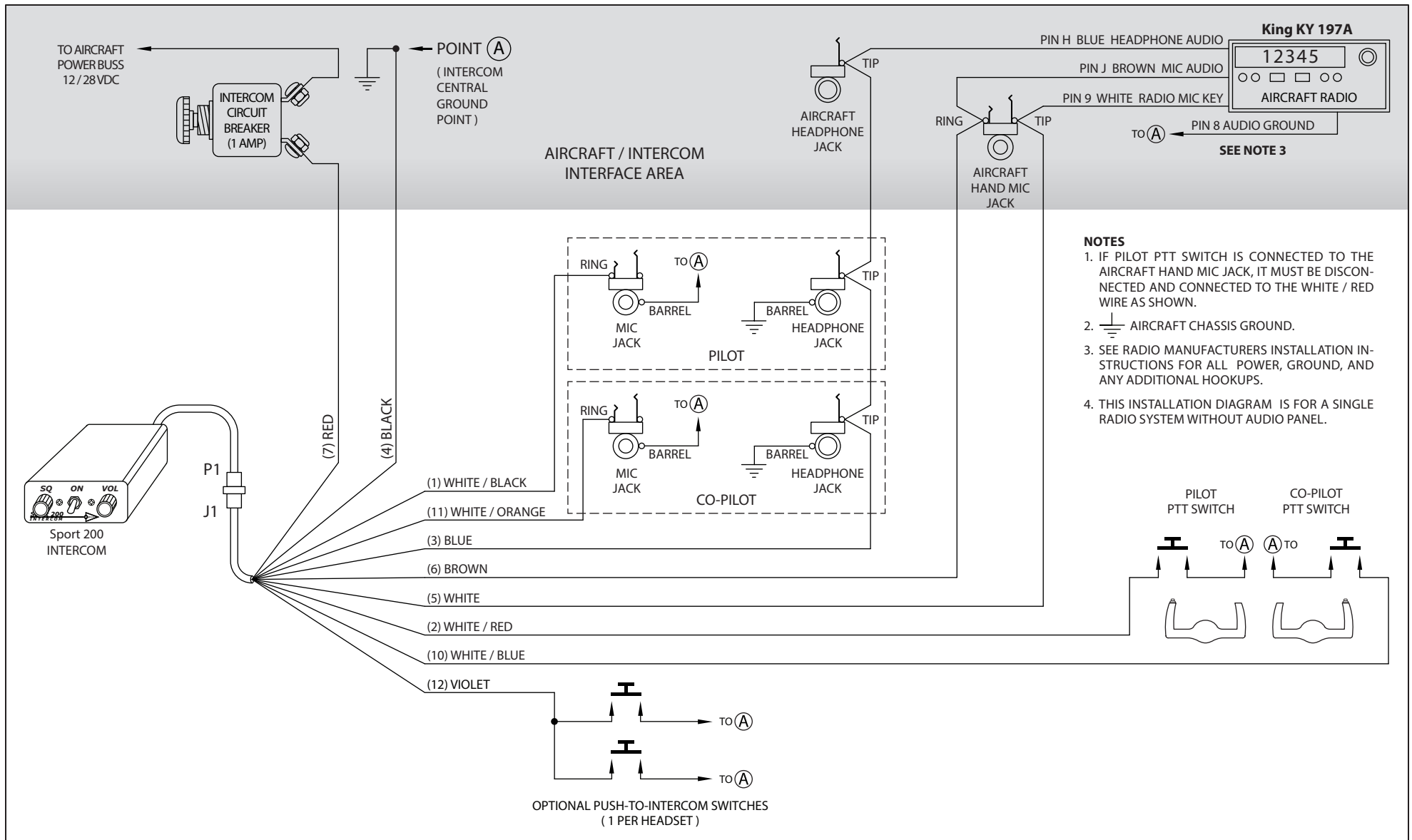
Sport 200 – King KY 197A Radio Installation Wiring Diagram
