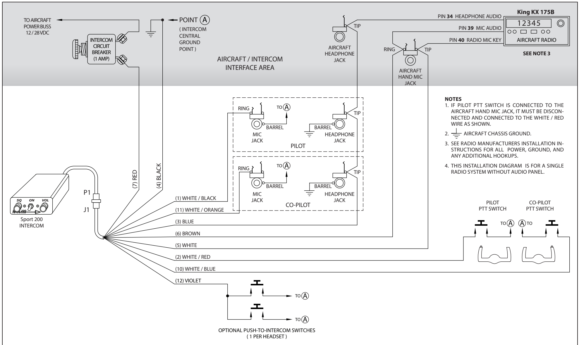
Sport 200 – King KX 175B Radio Installation Wiring Diagram
