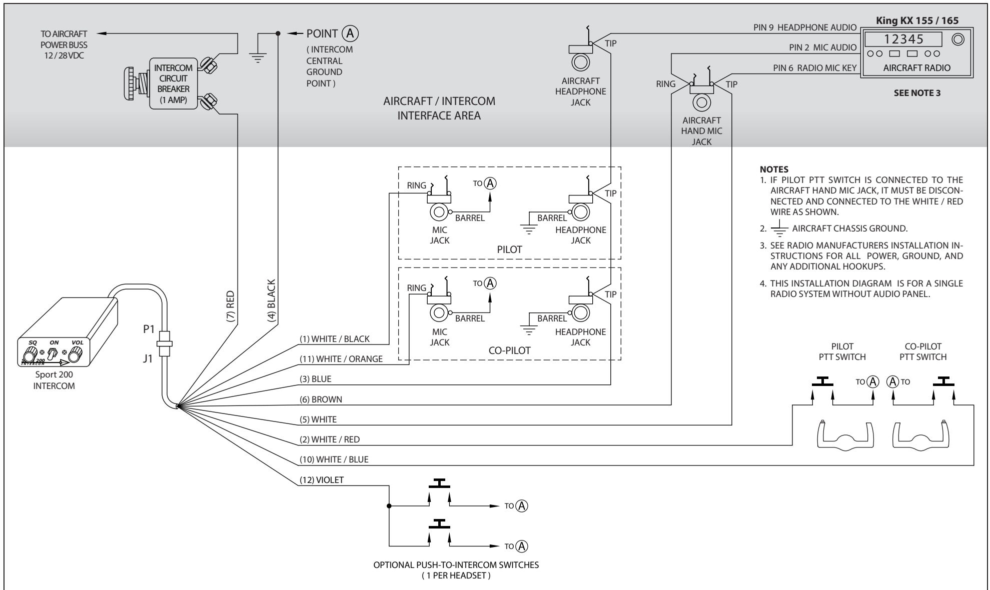
Sport 200 – King KX 155 / 165 Radio Installation Wiring Diagram
