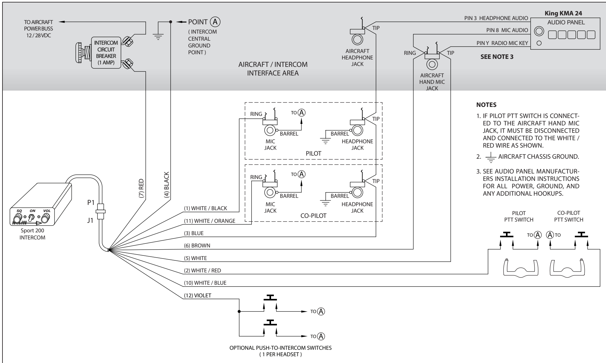
Sport 200 – King KMA 24 Audio Panel Installation Wiring Diagram
