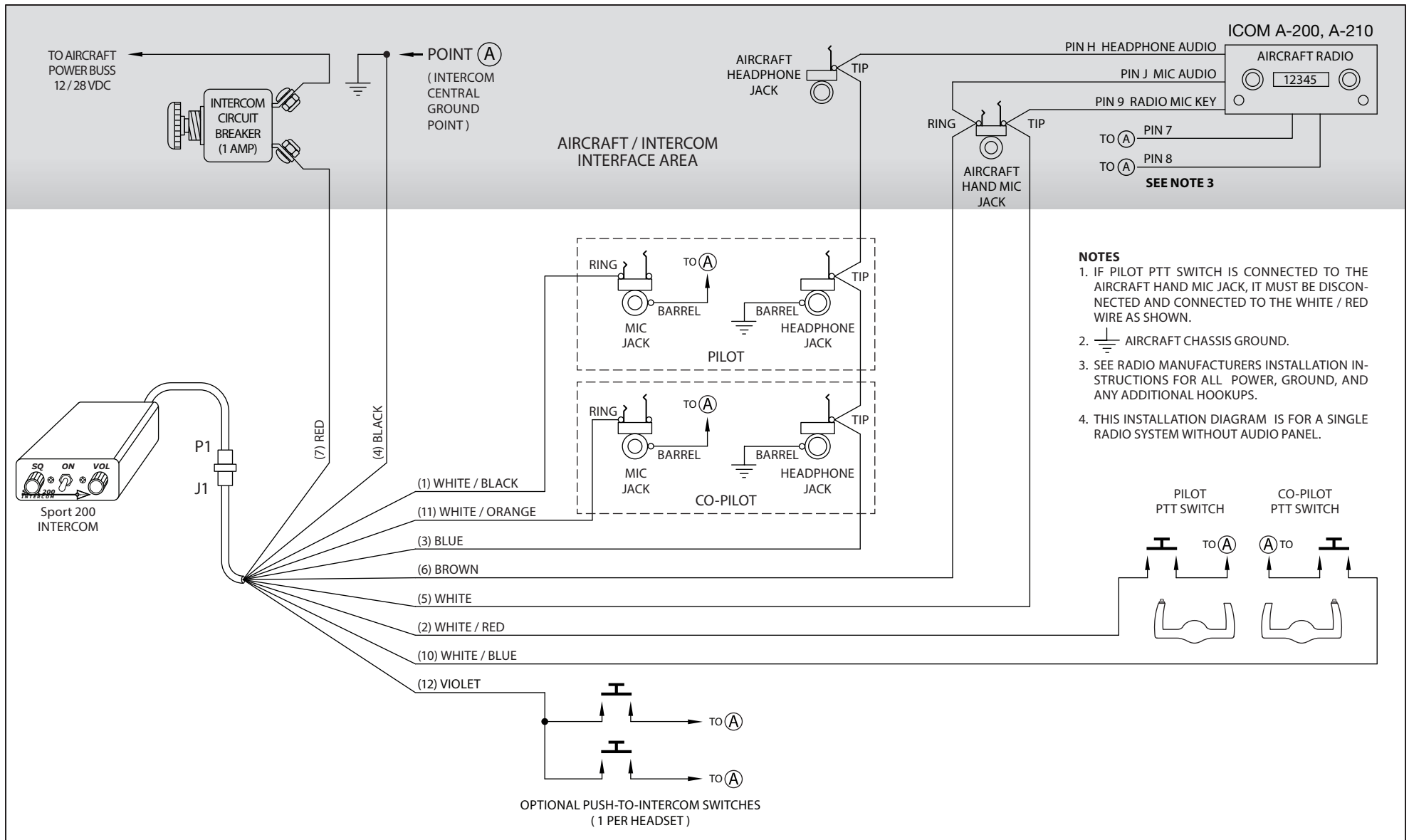
Sport 200 – ICOM A-200, A-210 Radio Installation Wiring Diagram
