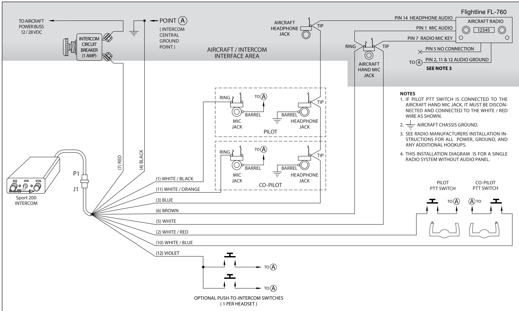
Sport 200 – Flightline FL-760 Radio Installation Wiring Diagram
