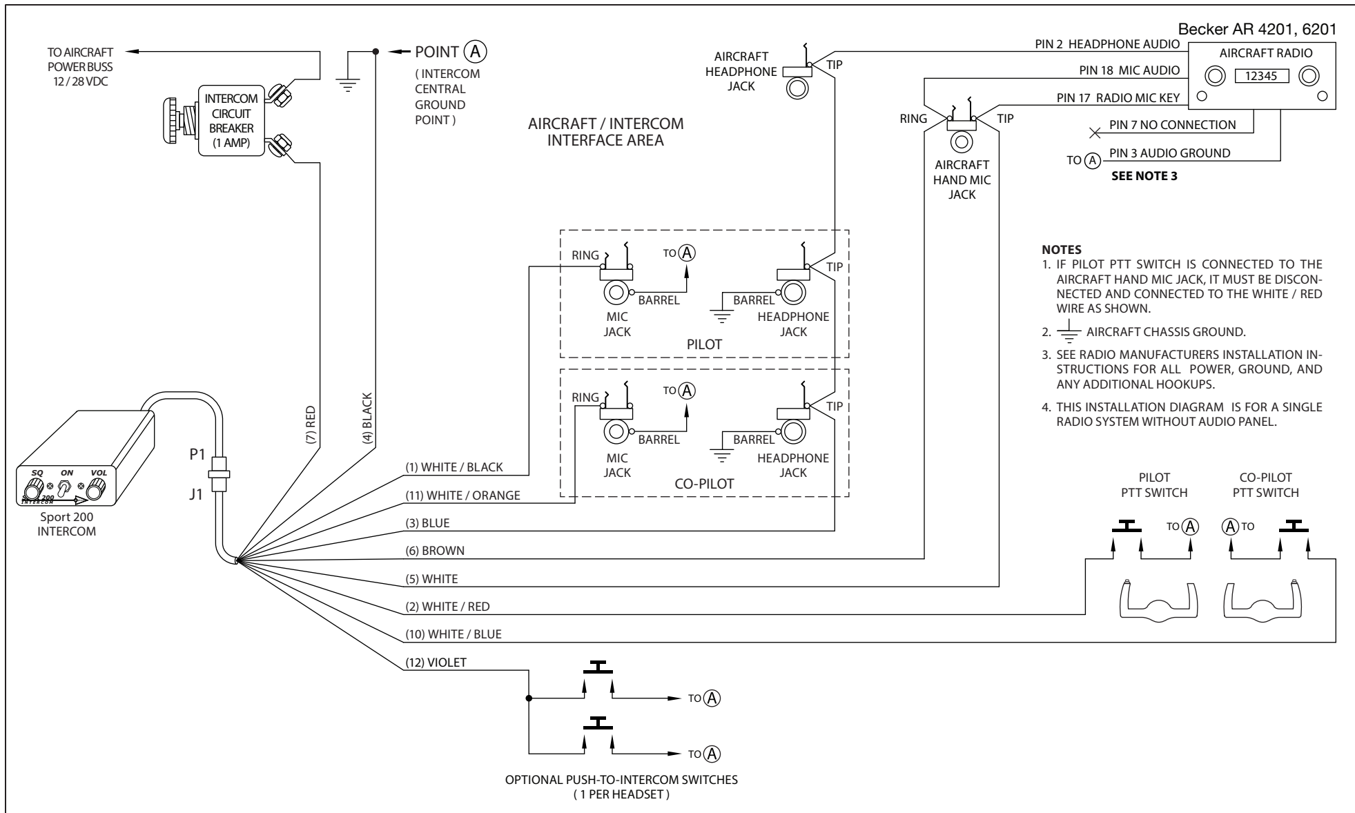
Sport 200 – Becker AR 4201, 6201 Radio Installation Wiring Diagram
