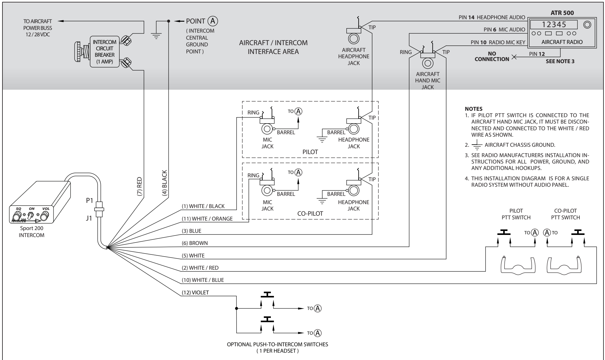
Sport 200 – Filser Electronic ATR 500 Radio Installation Wiring Diagram
