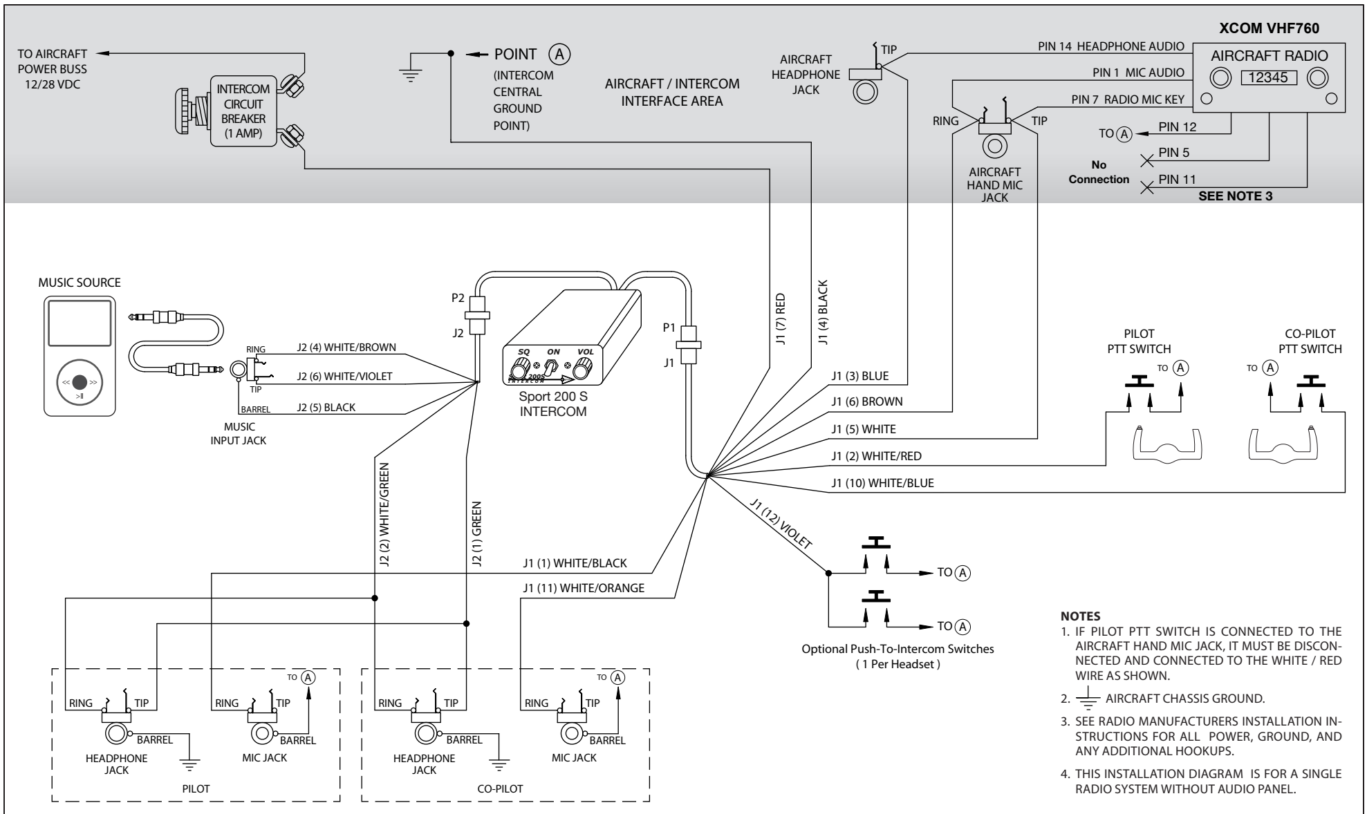
Sport 200S – XCOM VHF760 Radio Installation Wiring Diagram
