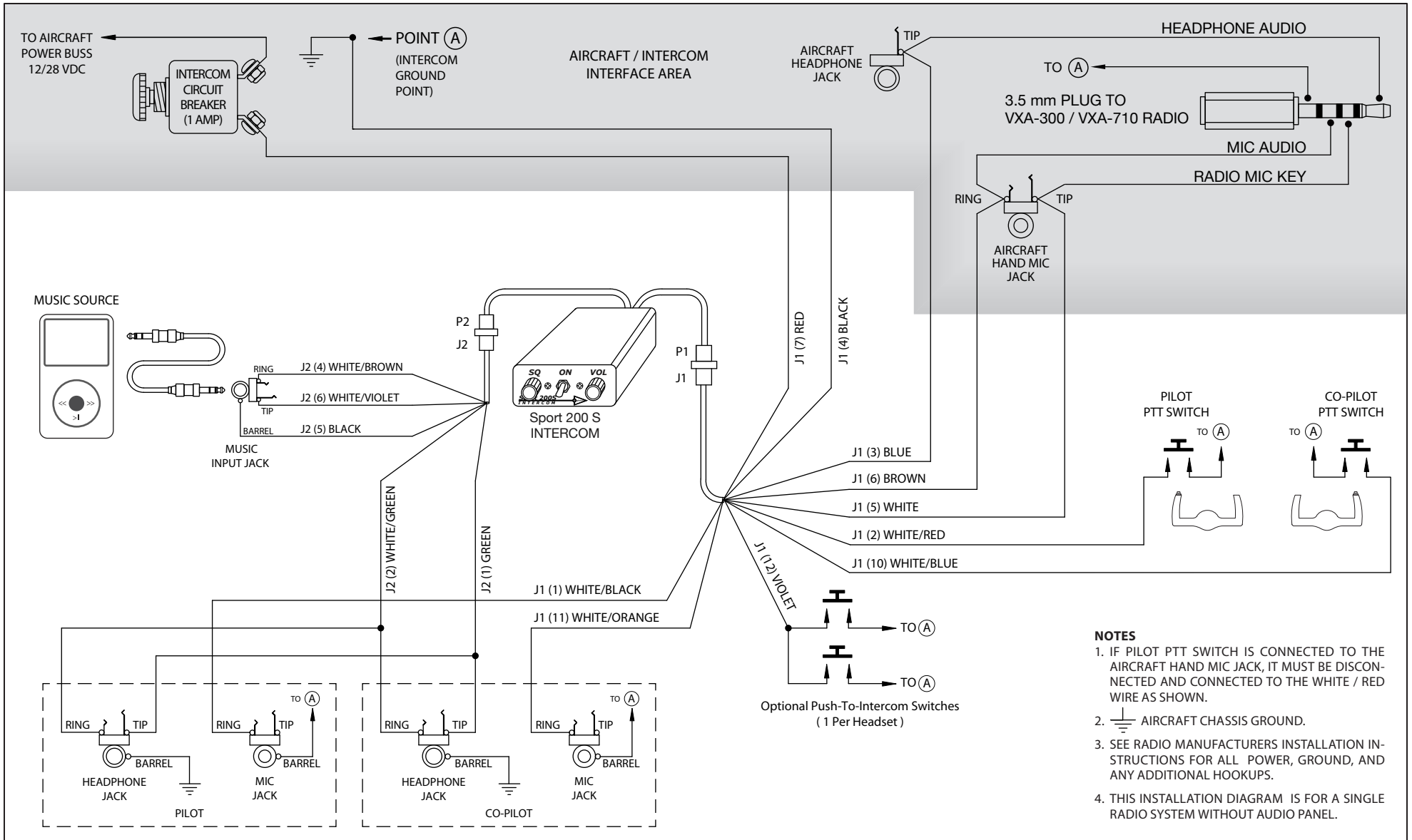
Sport 200S – Vertex Standard VXA-300 / VXA-710 Radio Installation Wiring Diagram
