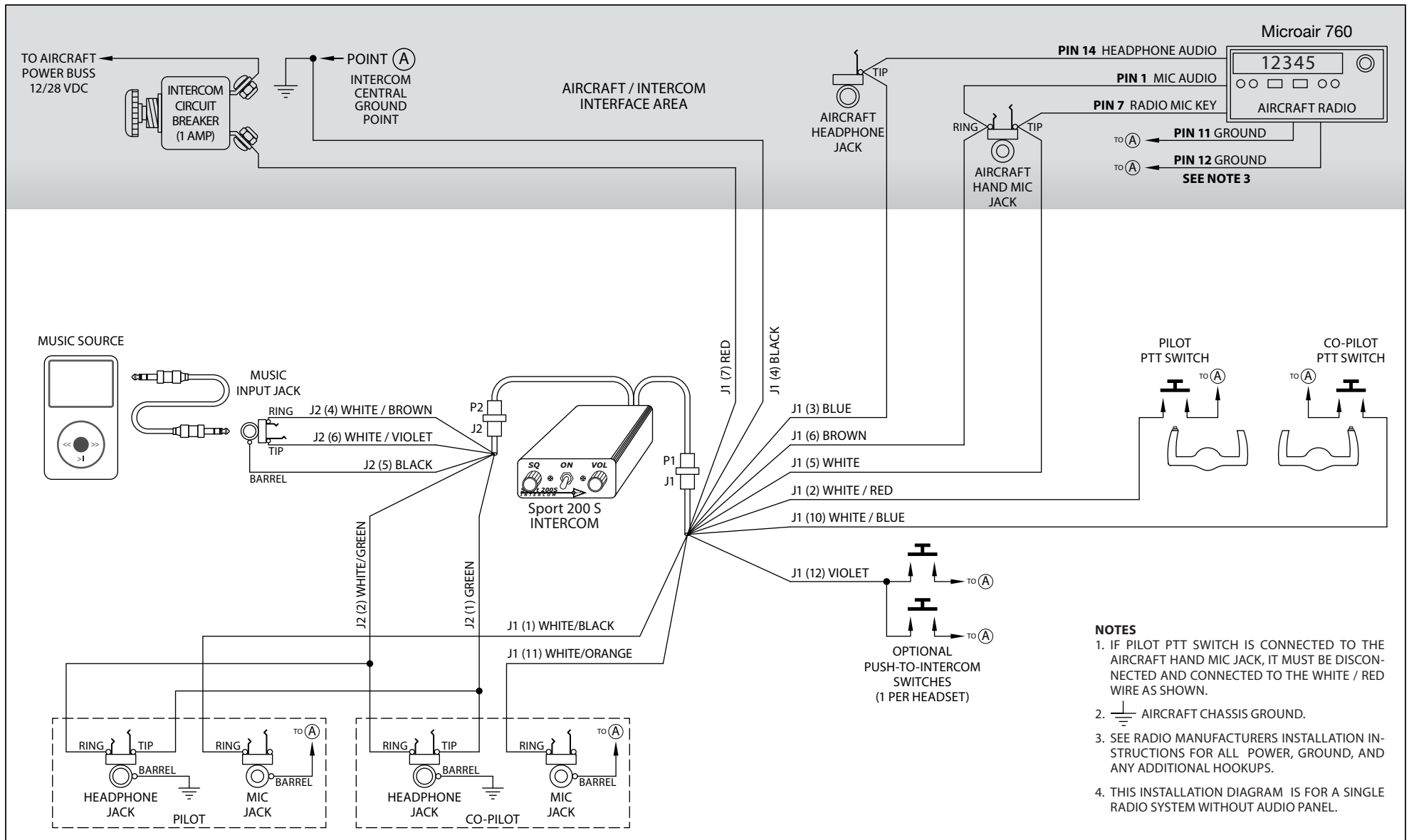
Sport 200S – Microair 760 Radio Installation Wiring Diagram
