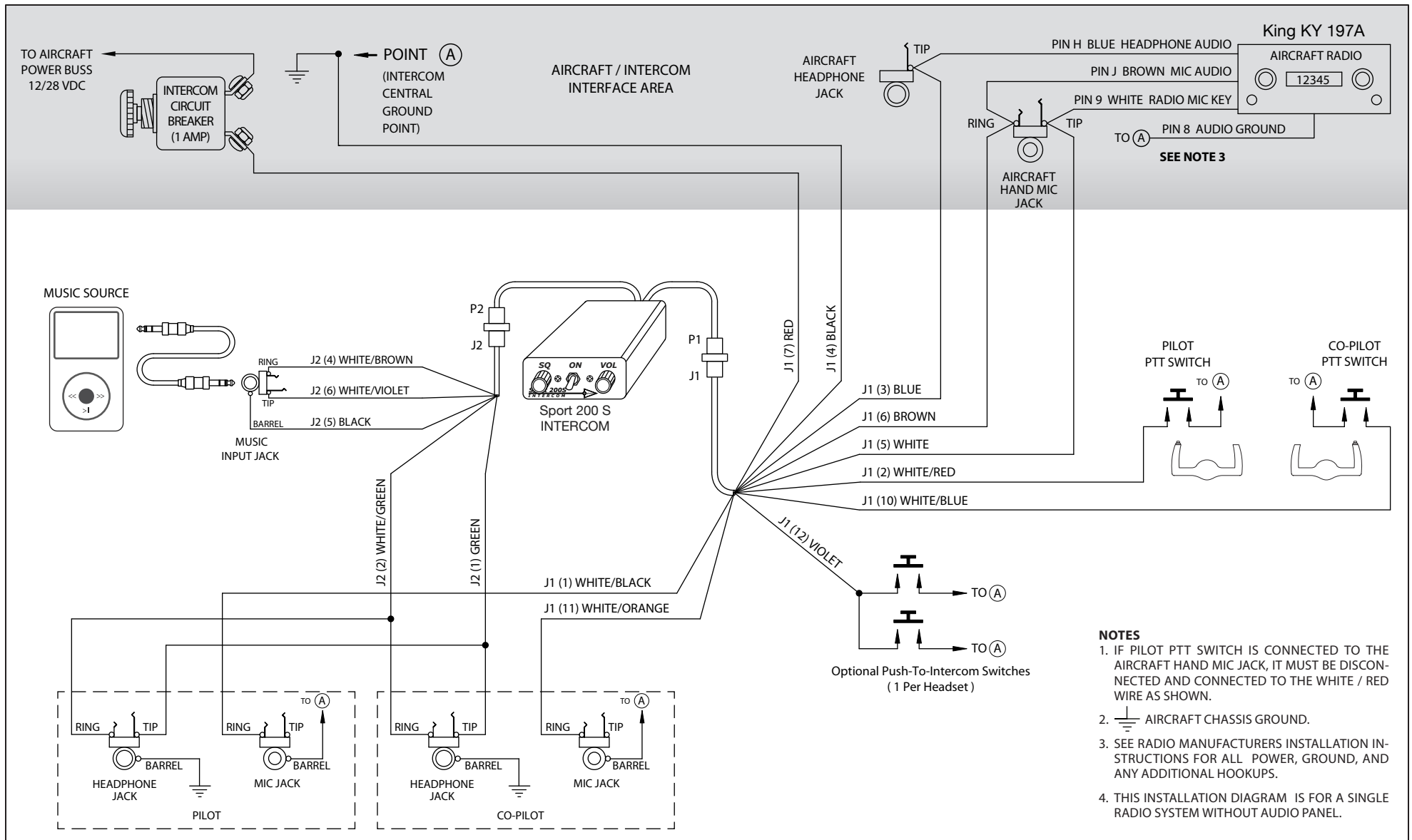
Sport 200S – King KY 197A Radio Installation Wiring Diagram
