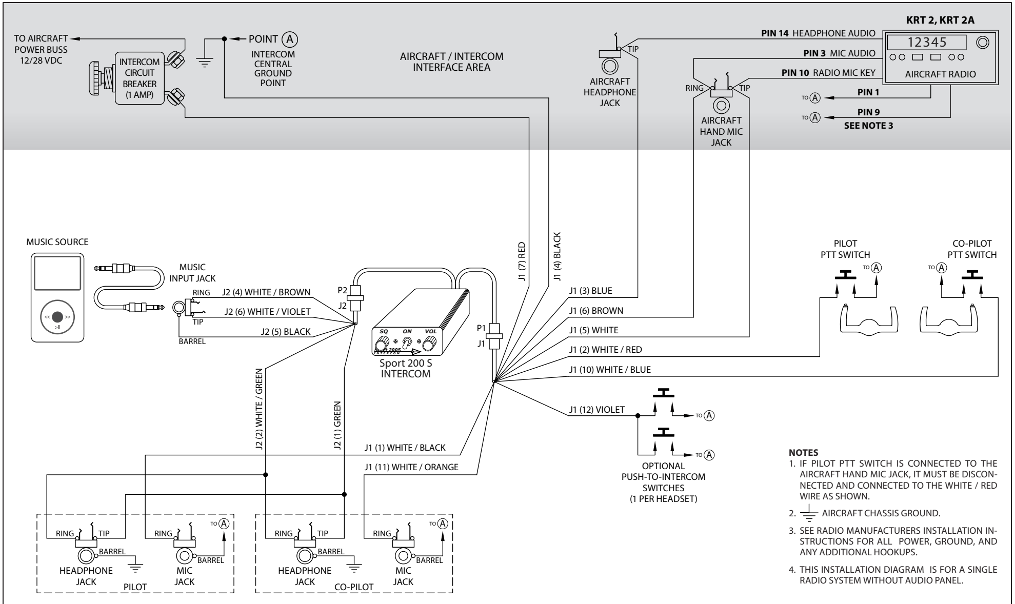
Sport 200S – KRT 2, KRT 2A Radio Installation Wiring Diagram
