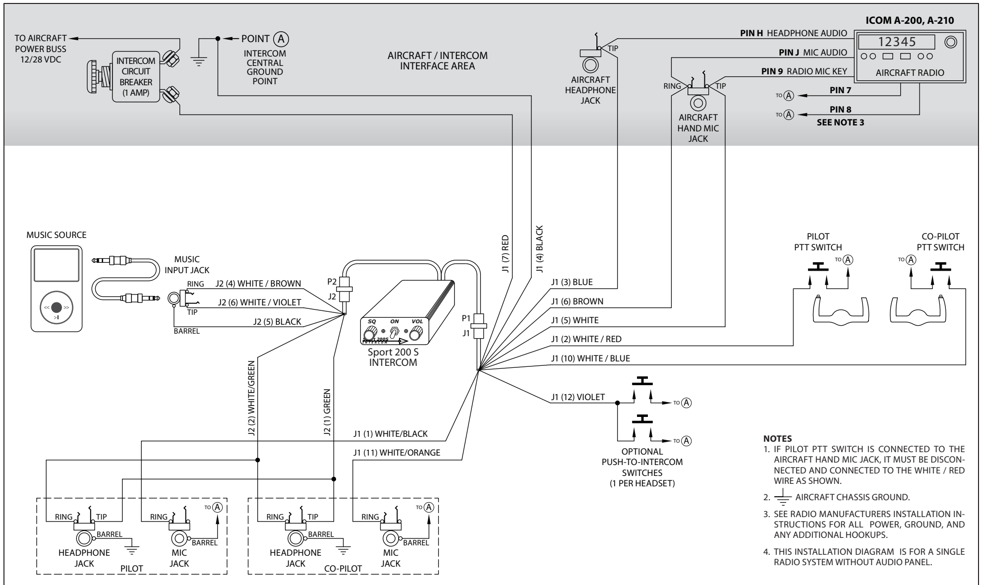
Sport 200S – ICOM A-200, A-210 Radio Installation Wiring Diagram
