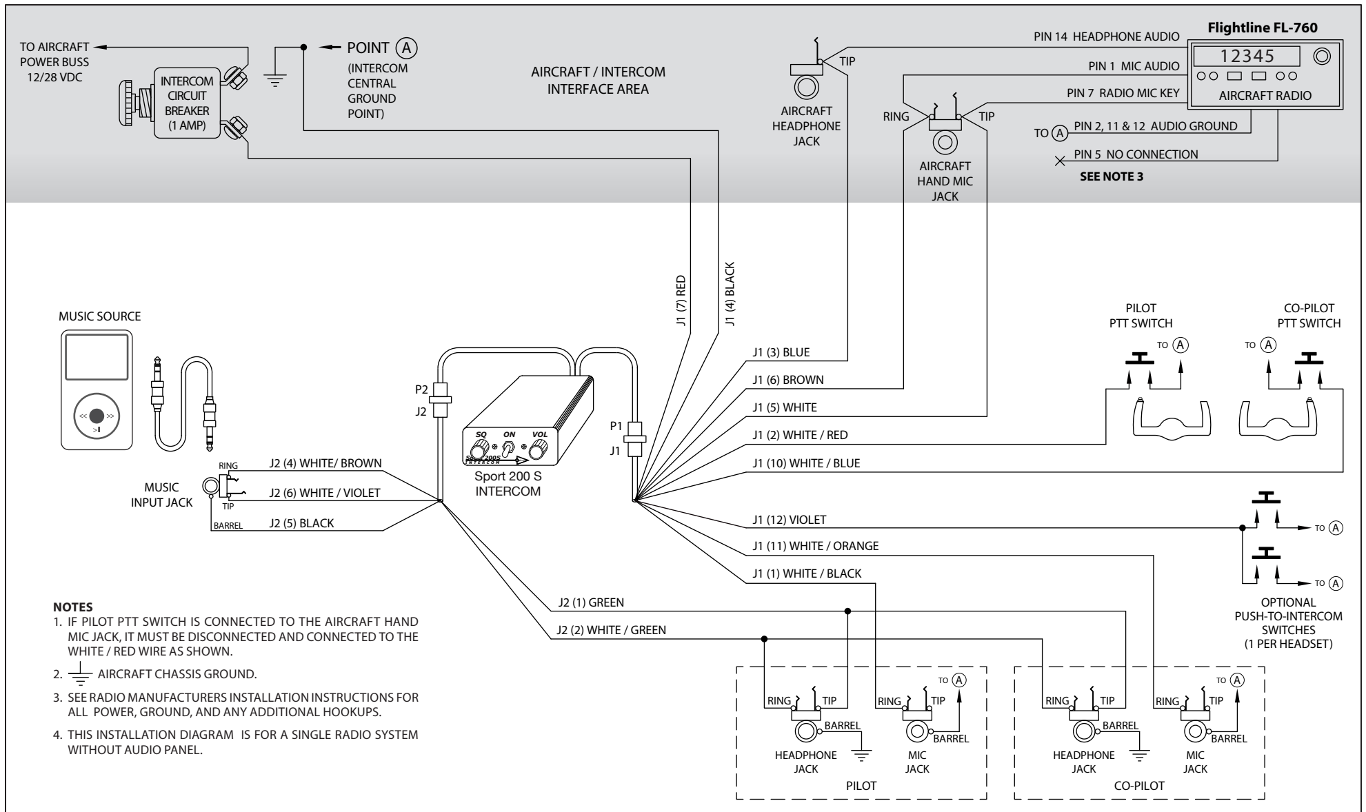
Sport 200S – Flightline FL-760 Radio Installation Wiring Diagram
