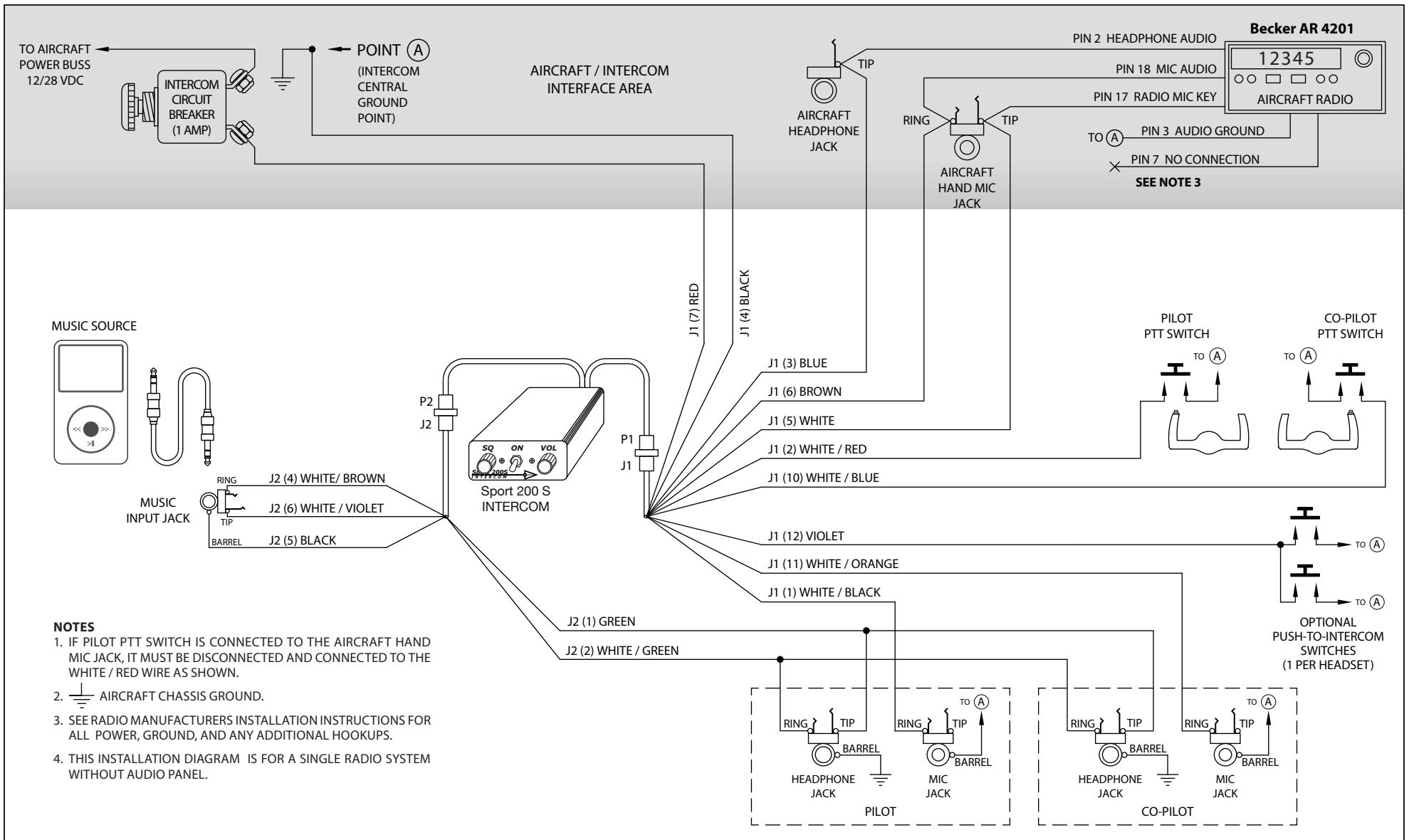
Sport 200S – Becker AR 4201 Radio Installation Wiring Diagram
