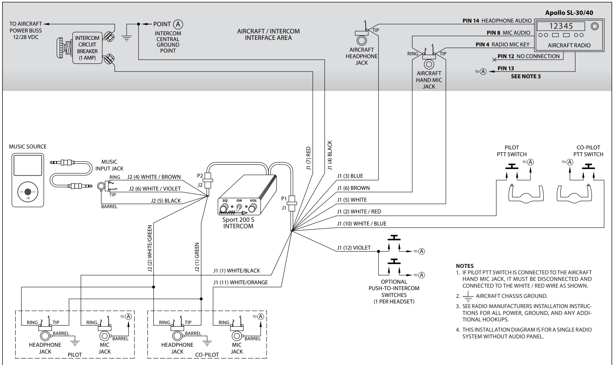
Sport 200S - Apollo SL-30 / 40 Radio Installation Wiring Diagram
