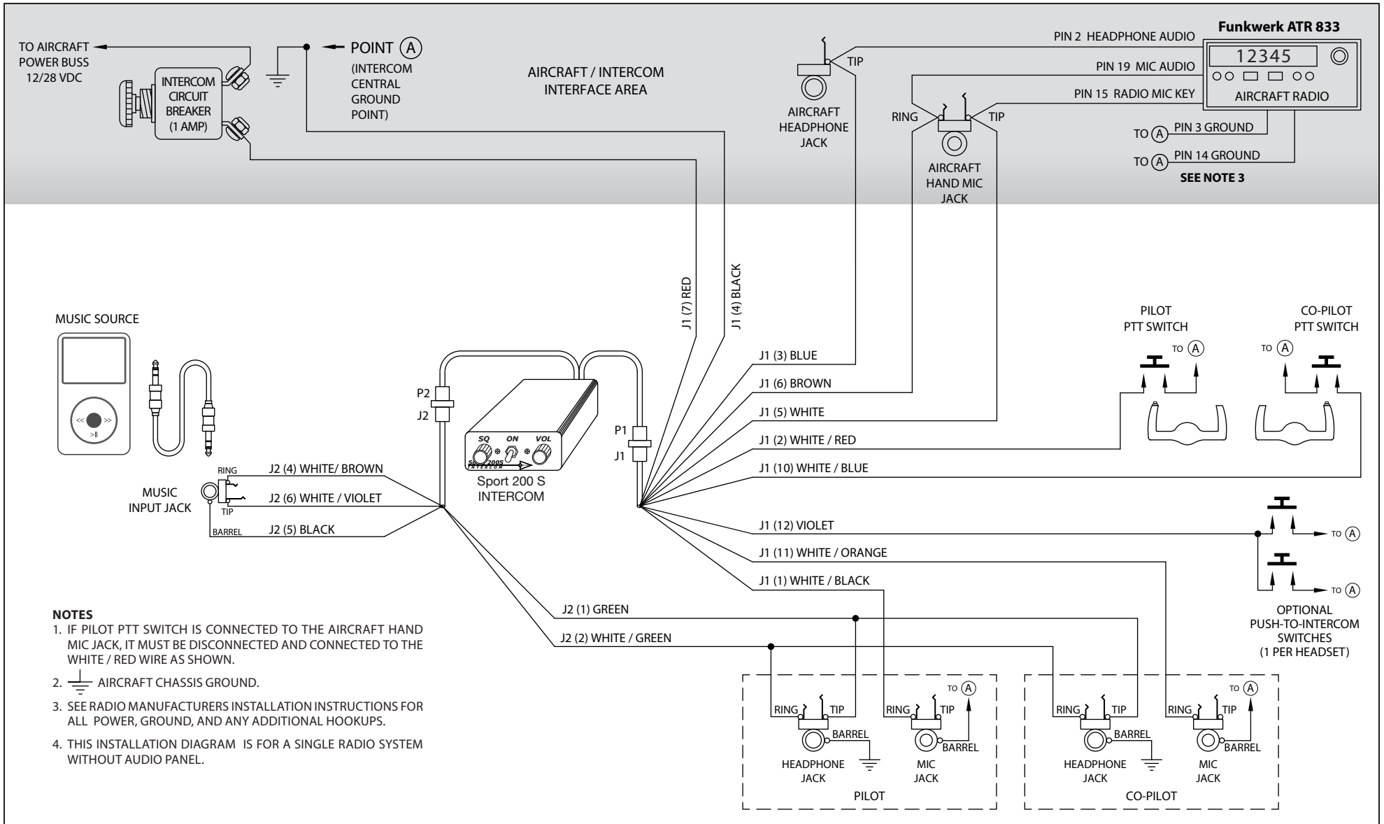
Sport 200S - Funkwerk ATR 833 Radio Installation Wiring Diagram
