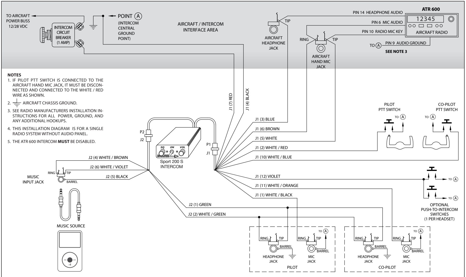
Sport 200S – Filser Electronic ATR 600 Radio Installation Wiring Diagram
