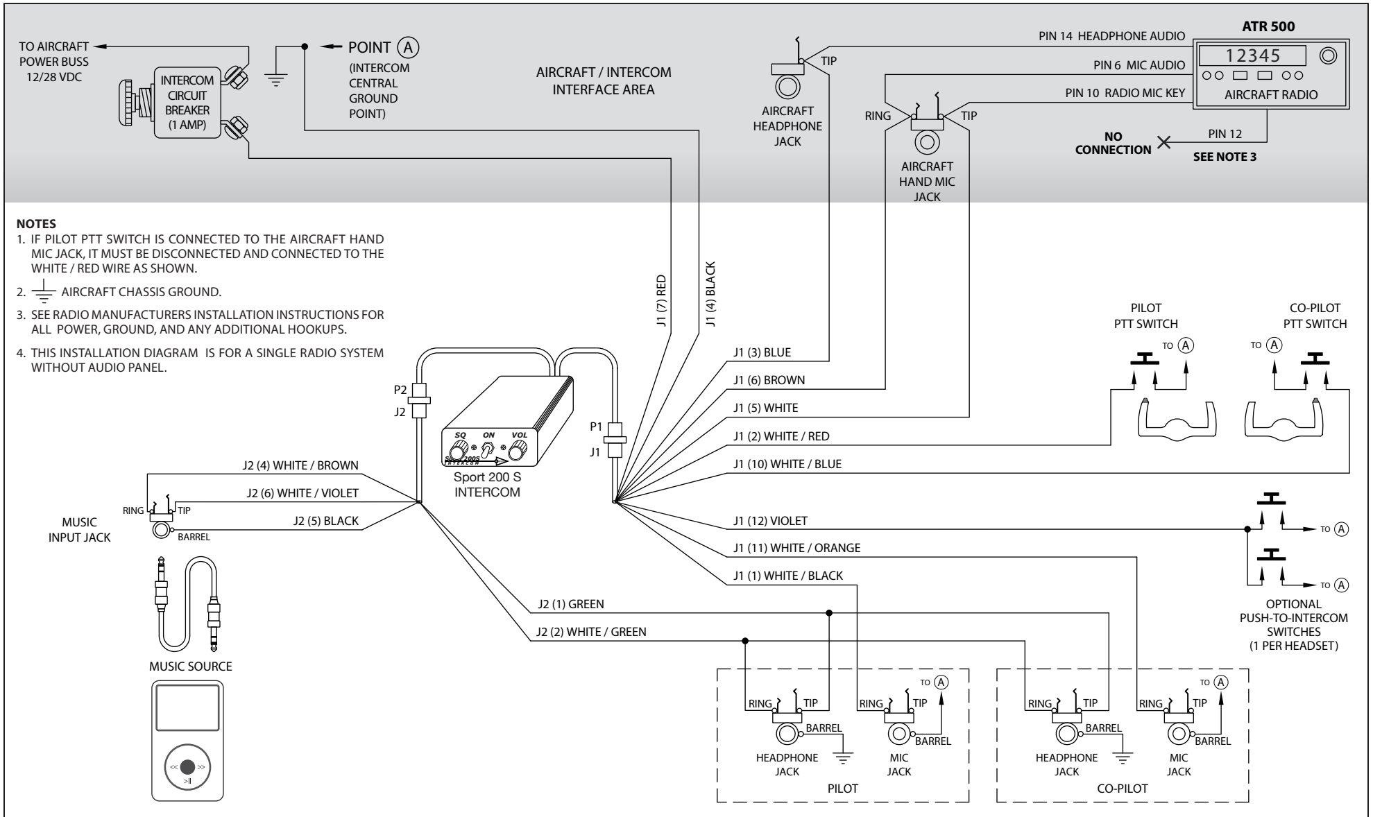
Sport 200S – Filser Electronic ATR 500 Radio Installation Wiring Diagram
