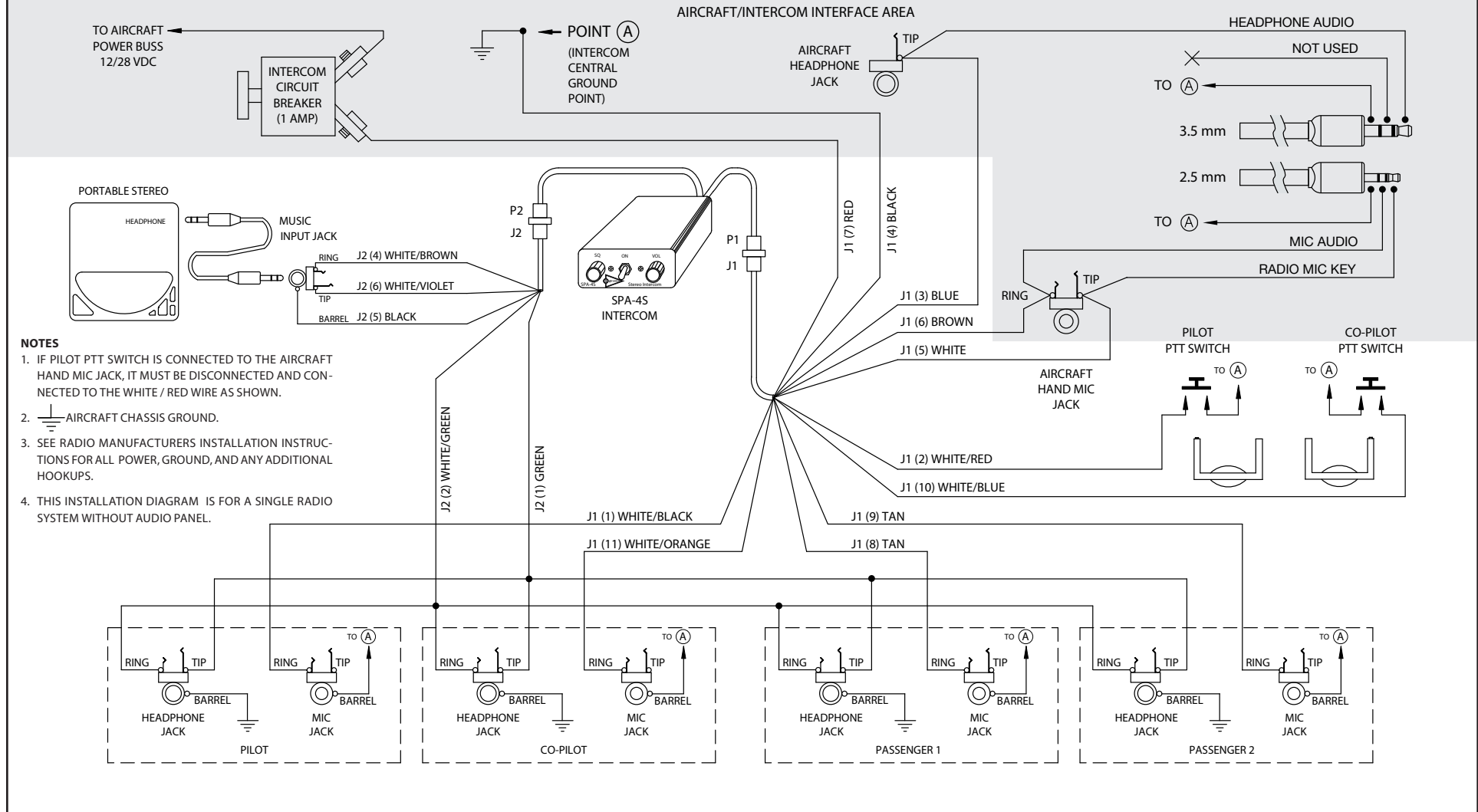
SPA-4S – ICOM A3, A6, A22, A24 Radio Installation Wiring Diagram
