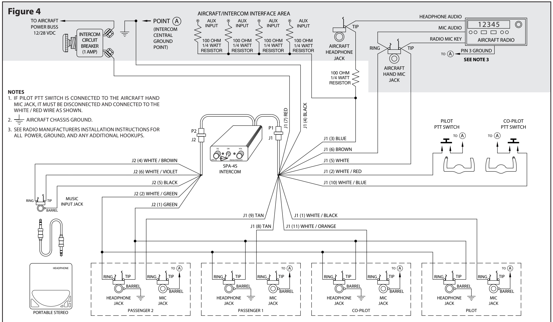
SPA-4S – AUX Audio Inputs Installation Wiring Diagram
