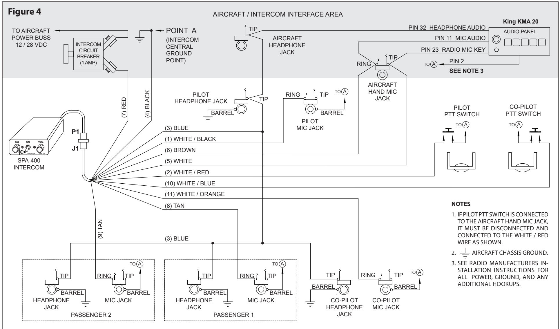
SPA-400 – King KMA 20 Audio Panel Installation Wiring Diagram
