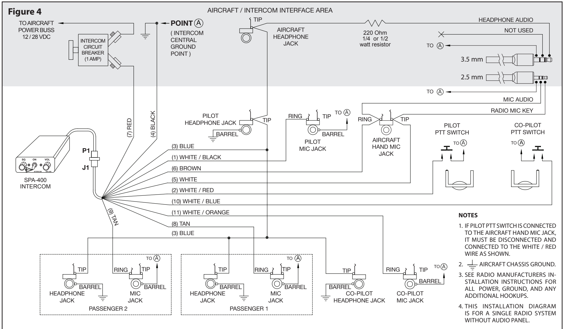
SPA-400 – ICOM A3, A6, A22, A24 Radio Installation Wiring Diagram
