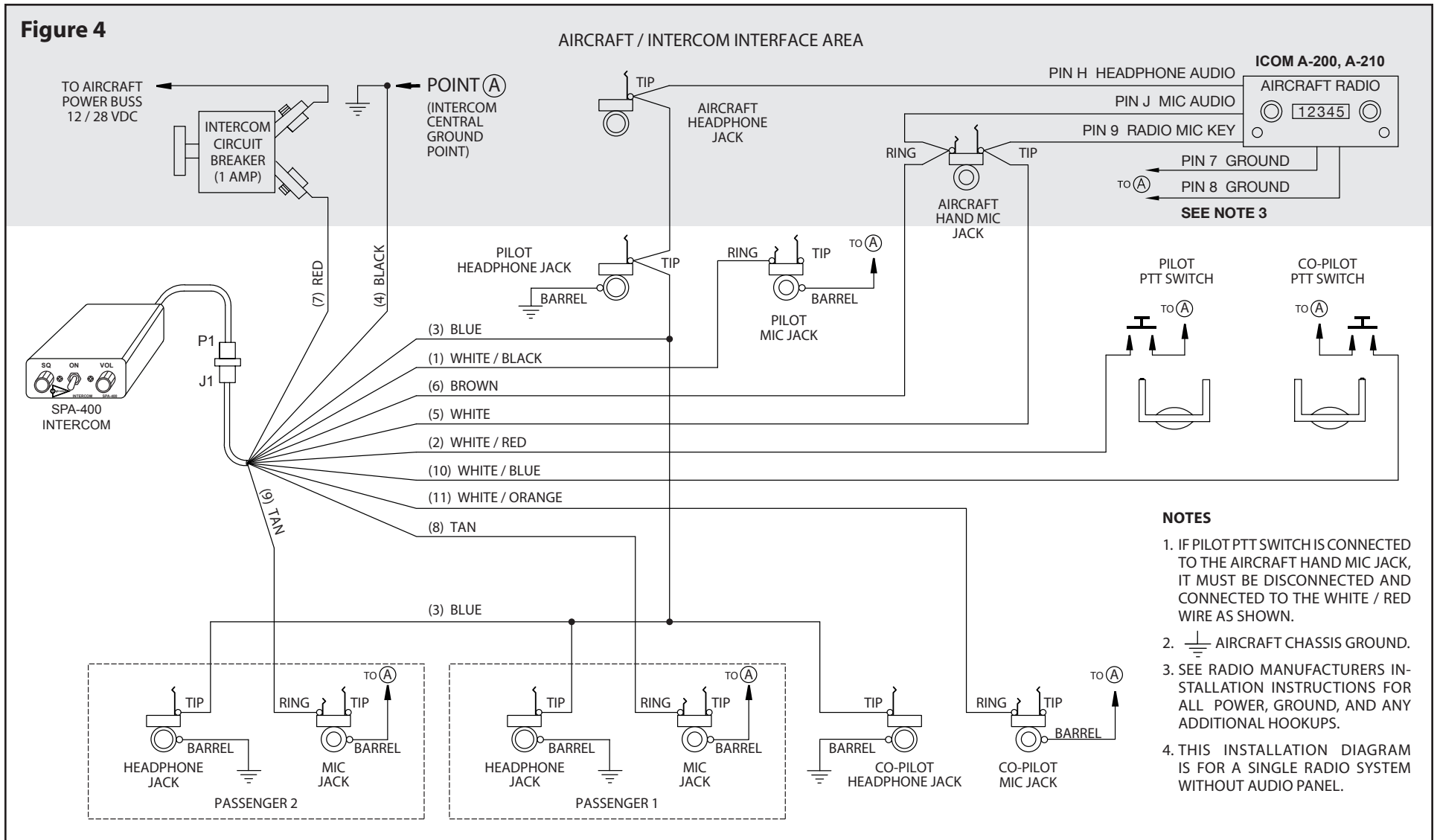
SPA-400 – ICOM A-200, A-210 Radio Installation Wiring Diagram
