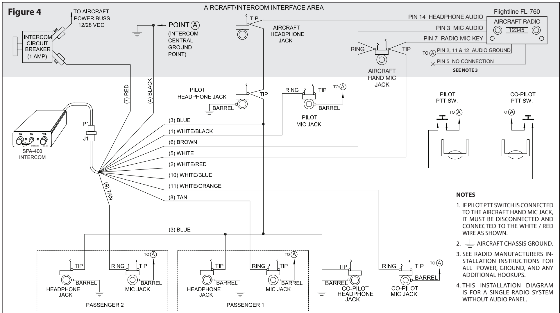
SPA-400 – Flightline FL-760 Radio Installation Wiring Diagram
