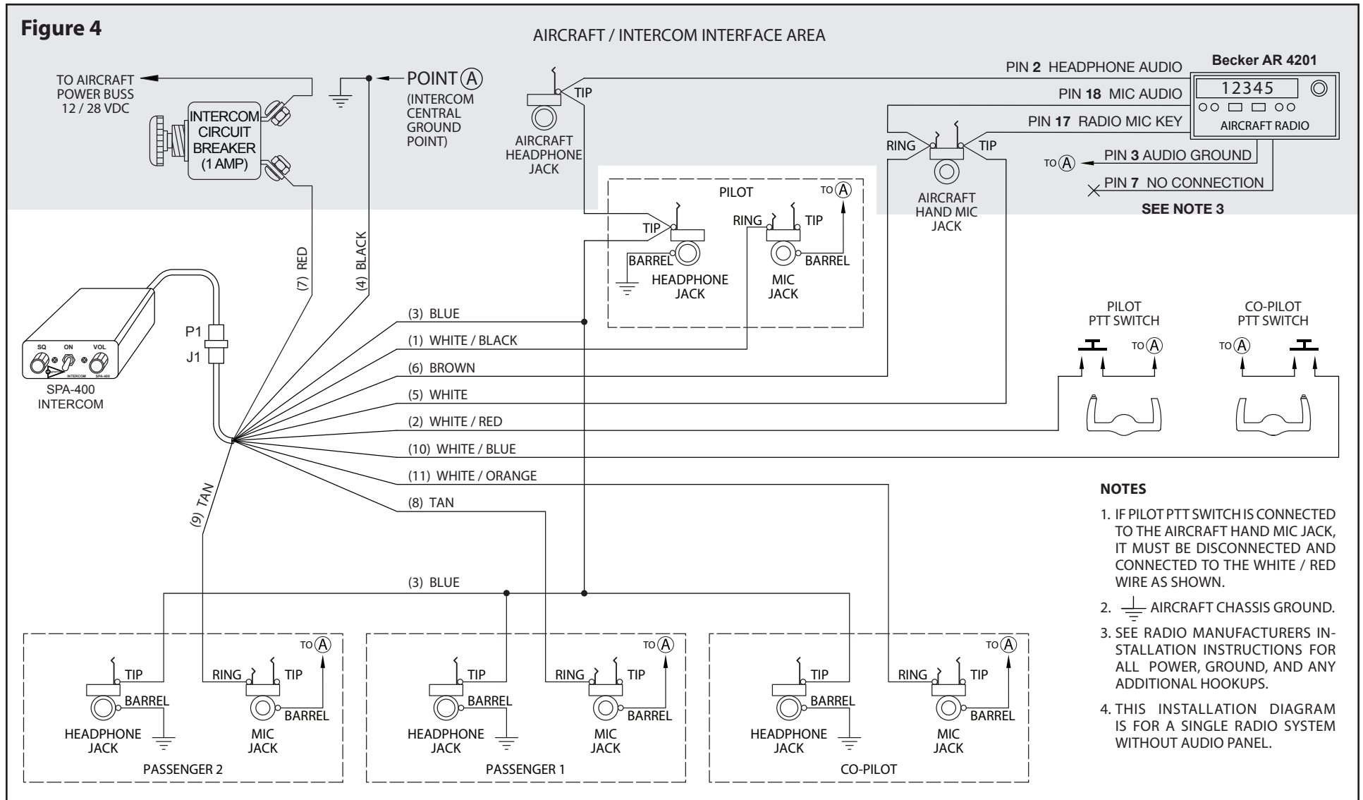
SPA-400 – Becker AR 4201 Radio Installation Wiring Diagram
