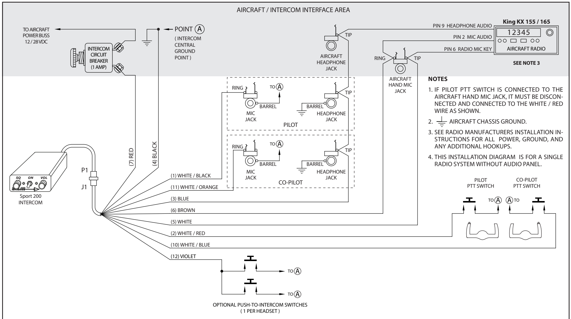
Sport 200 – King KX 155 / 165 Radio, Audio Amp Option Installation Wiring Diagram
