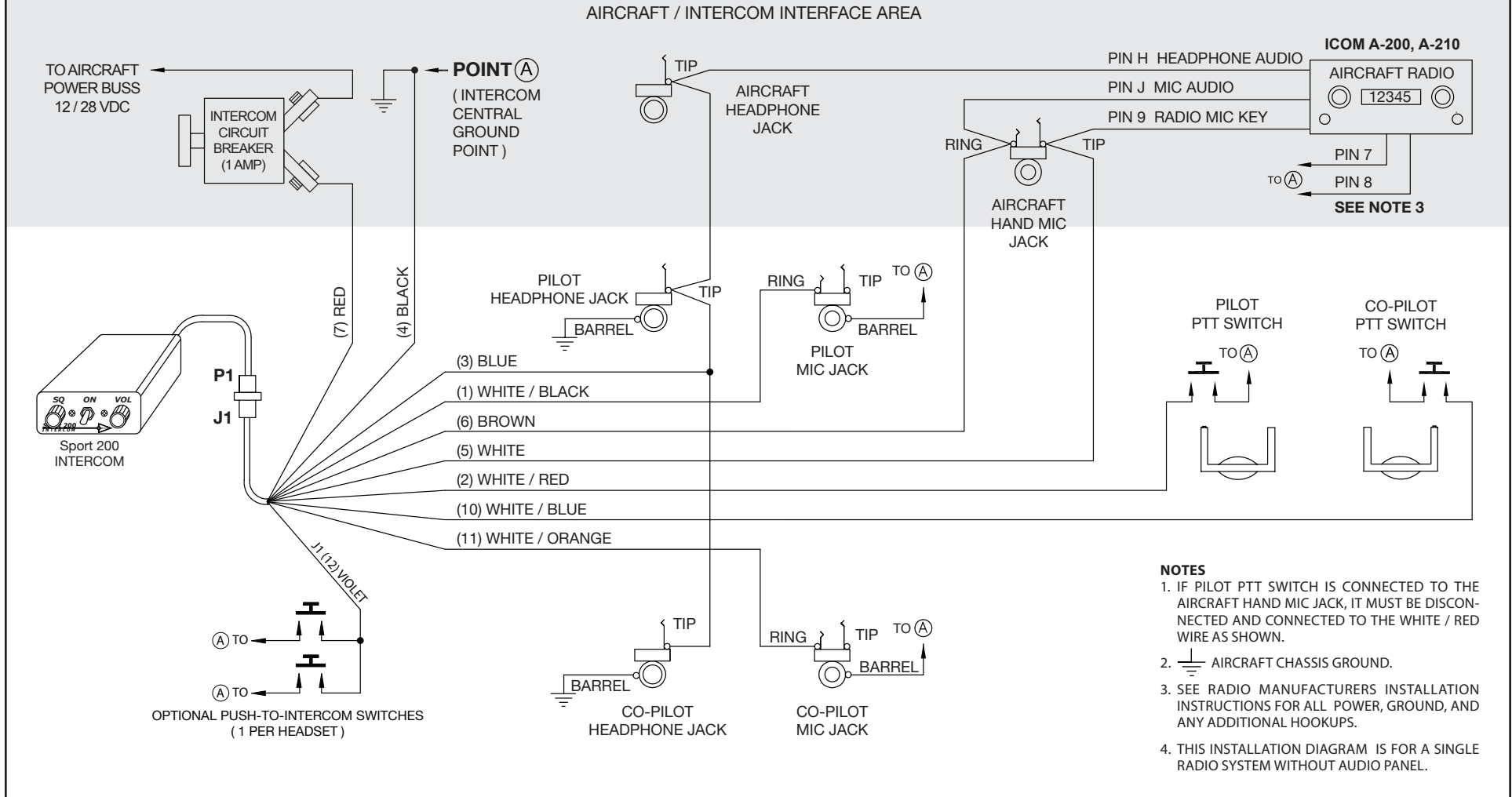
Sport 200 – ICOM A-200, A-210 Radio Installation Wiring Diagram
