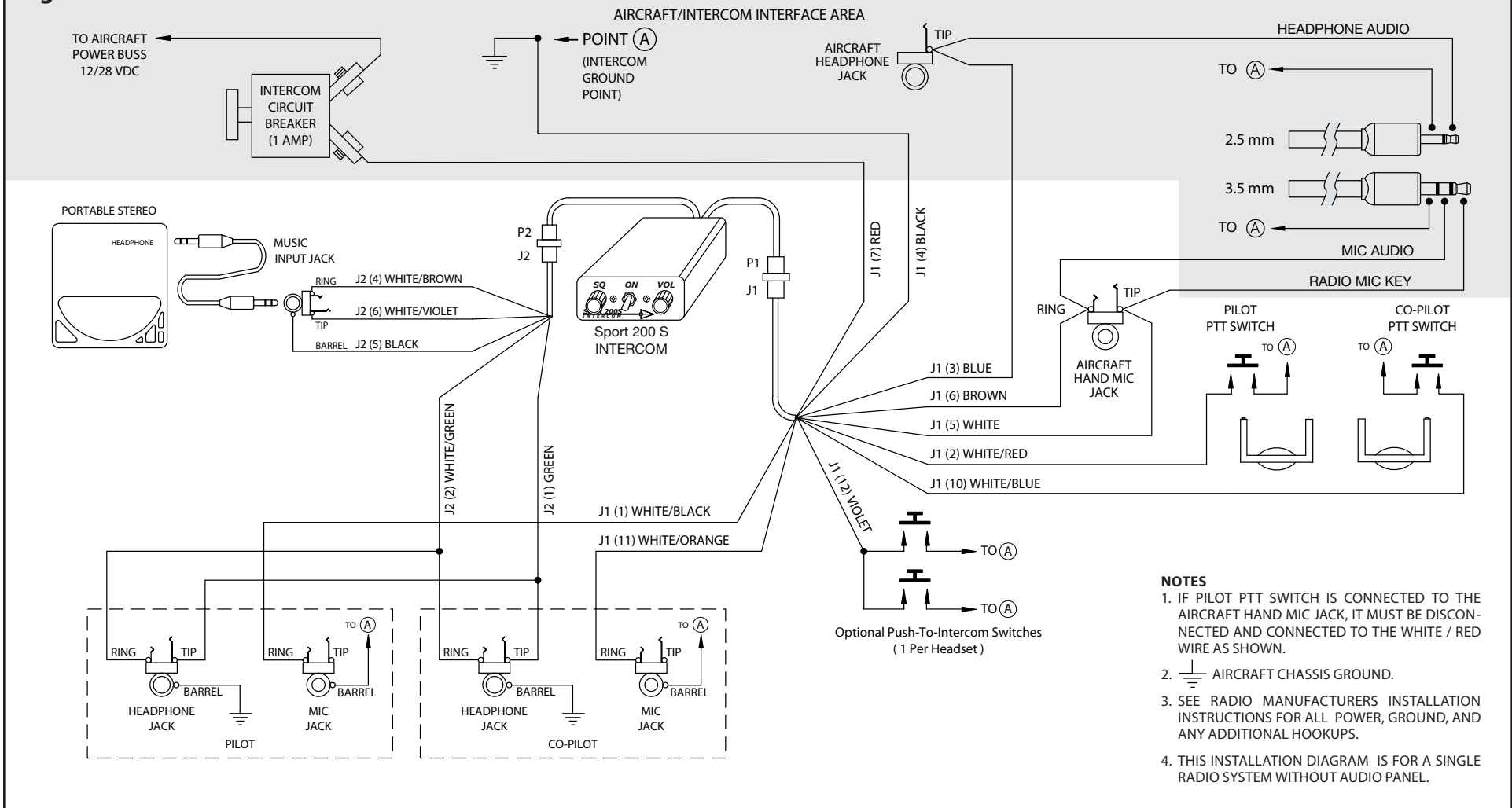
Sport 200S – Sporty's SP-200 Radio Installation Wiring Diagram
