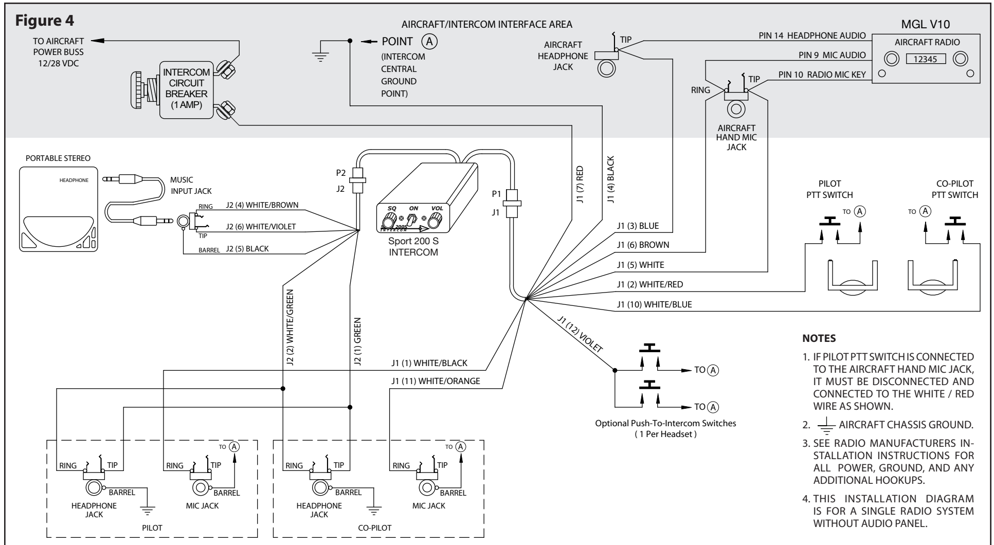
Sport 200S – MGL V10 Radio Installation Wiring Diagram
