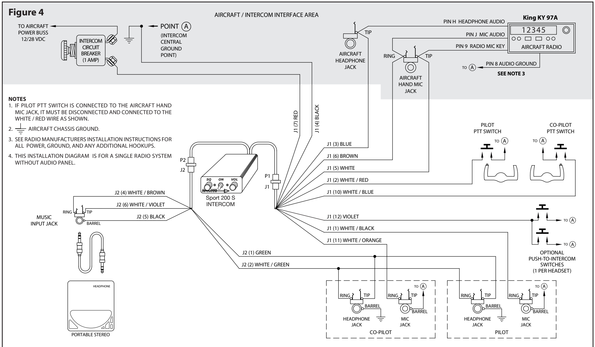
Sport 200S – King KY 97A Radio Installation Wiring Diagram
