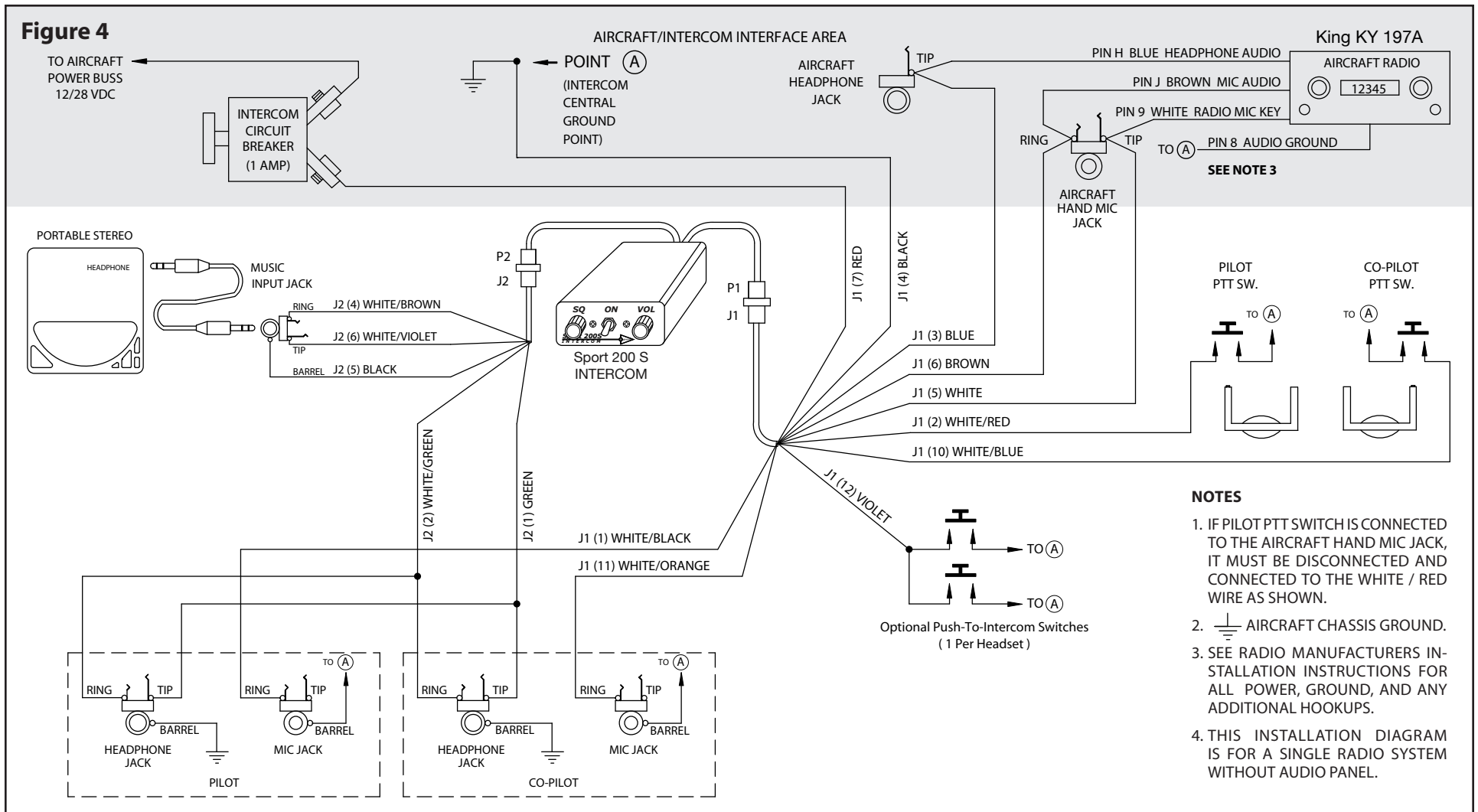
Sport 200S – King KY 197A Radio Installation Wiring Diagram
