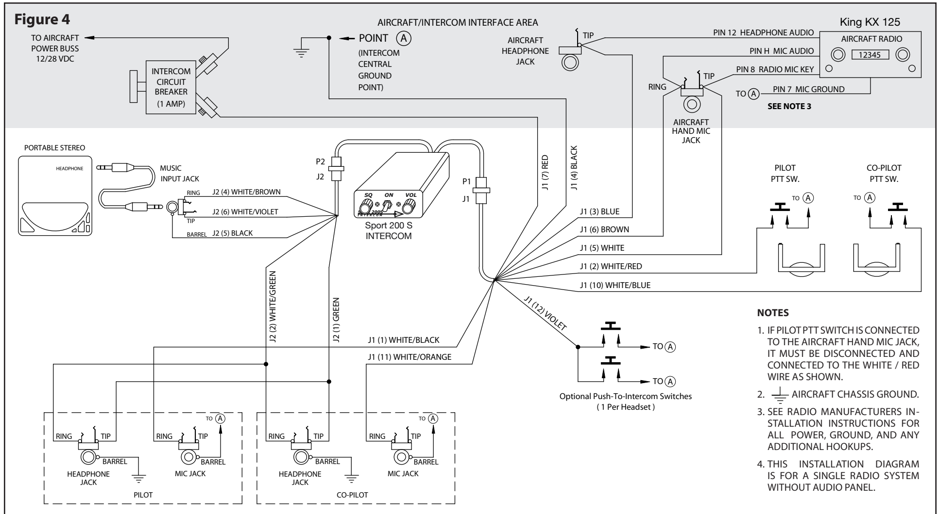
Sport 200S – King KX 125 Radio Installation Wiring Diagram
