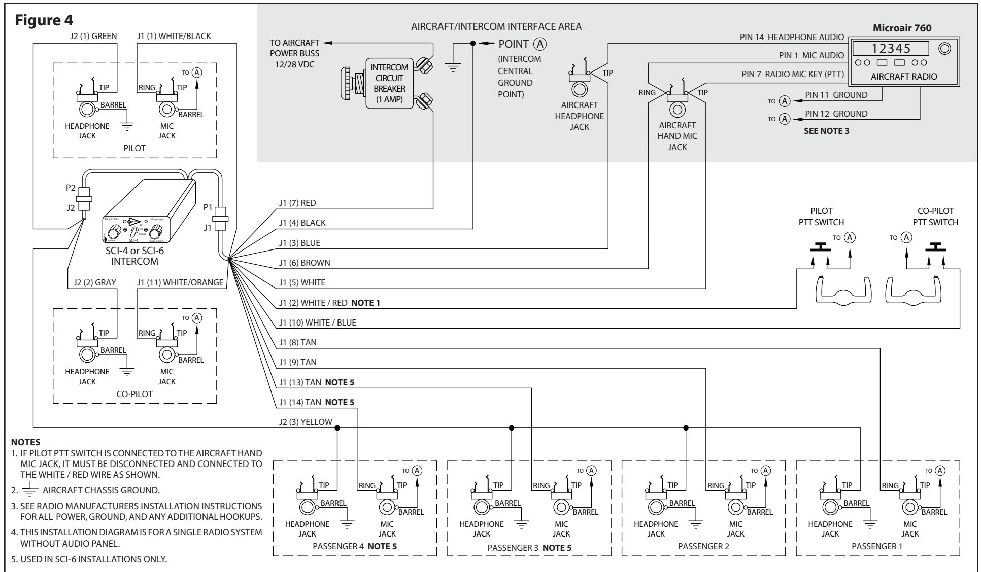
SCI-4 / SCI-6 – Microair 760 Radio Installation Wiring Diagram
