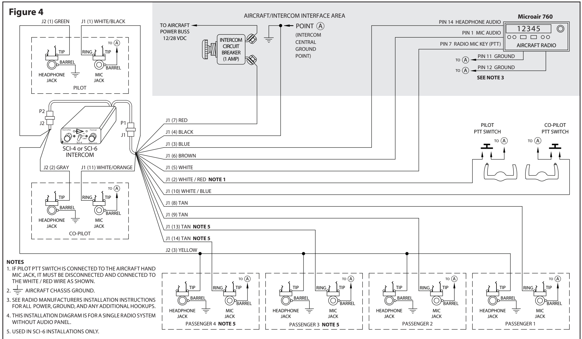
SCI-4 / SCI-6 – Microair 760 Radio (No Aircraft Jacks) Installation Wiring Diagram
